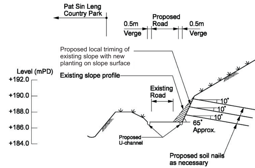
Typical Road Improvement Works at Section 8 - 8
