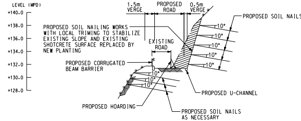
SECTION 5 SCALE 1:200 SK/005
