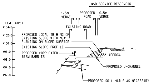
SECTION 4 SCALE 1:200 SK/005
