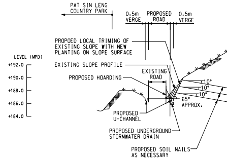
SECTION 8 SCALE 1:200 SK/005
