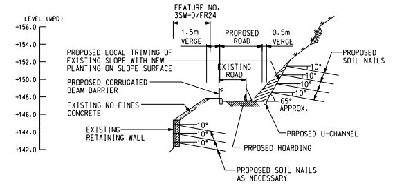
SECTION 6 SCALE 1:200 SK/005
