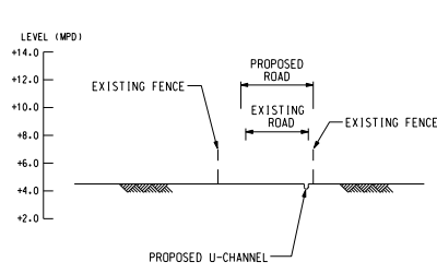
SECTION 1 SCALE 1:200 SK/005
