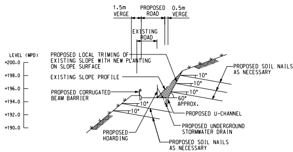
SECTION 7 SCALE 1:200 SK/005
