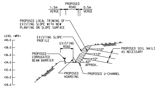
SECTION 2 SCALE 1:200 SK/005
