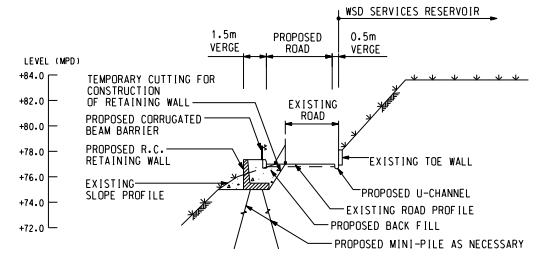
SECTION 3 SCALE 1:200 SK/005
