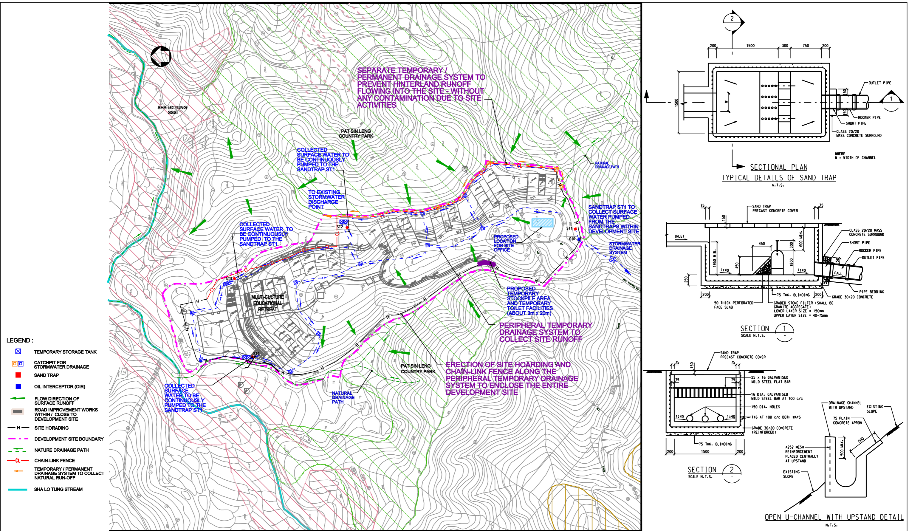
Figure 6.3 Temporary Drainage Layout Plan
