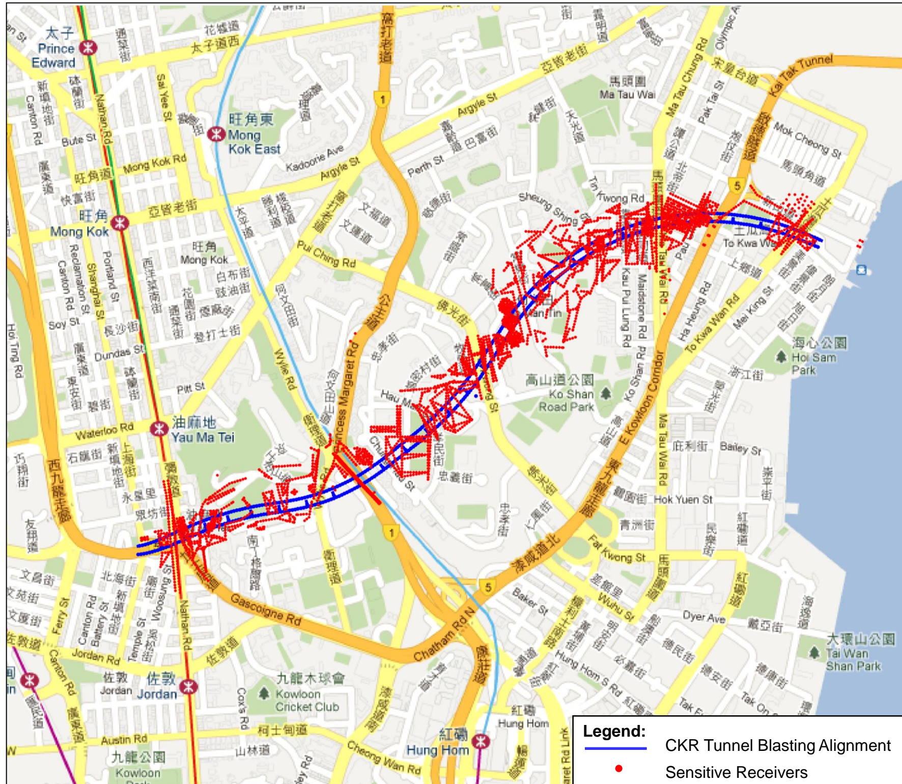
CKR Tunnel Blasting Alignment and Sensitive Receivers
