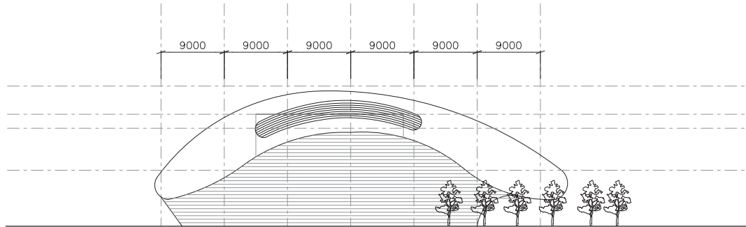
NORTH ELEVATION
