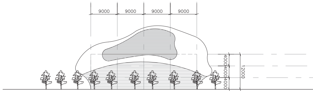
EAST ELEVATION
