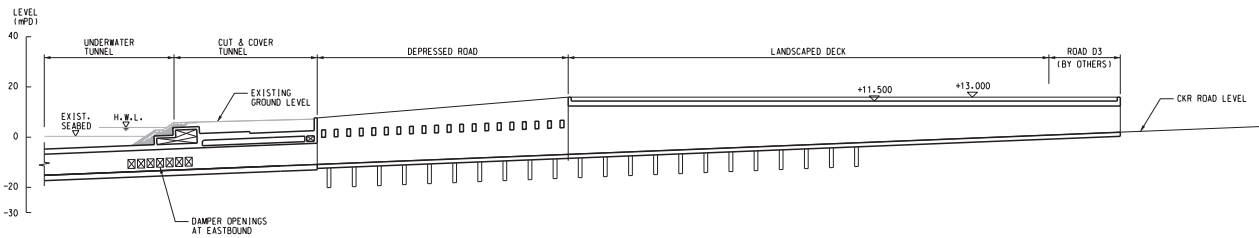
SECTION 1 SCALE 1:1000
