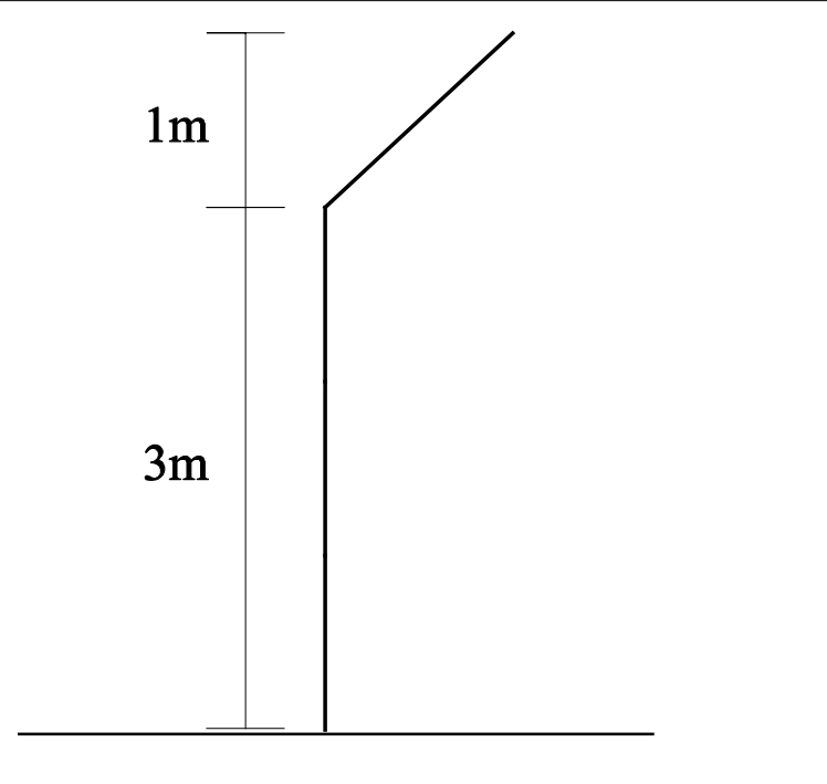
Temporary Noise Barrier (Cross Section X - X)
