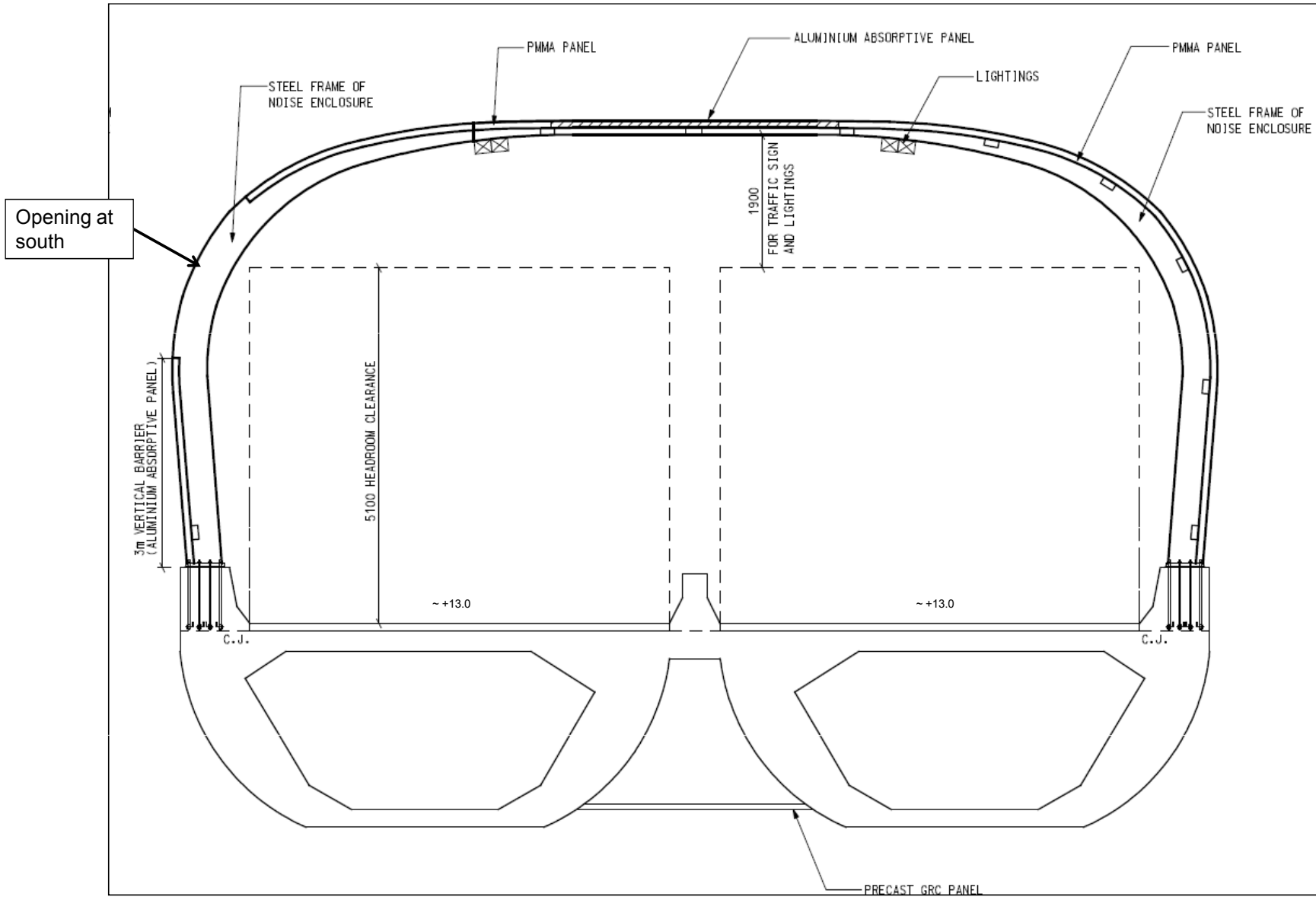
Section N - N
