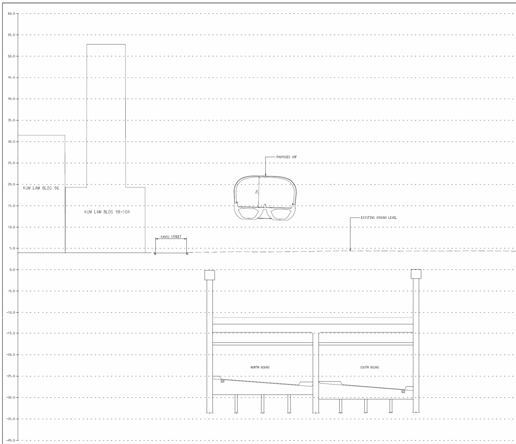
Section P - P
