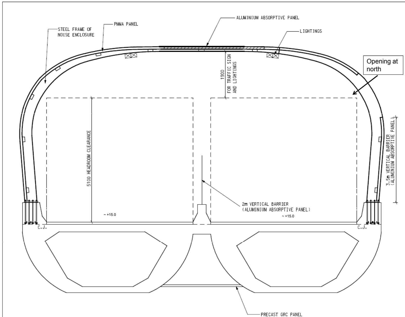
Section Q - Q
