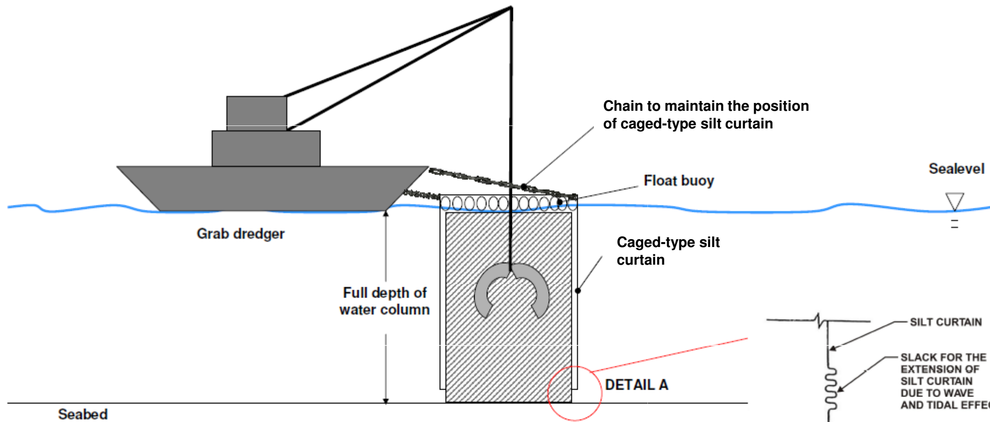
Additional Caged-Type Silt Curtain for Grab Dredgers
