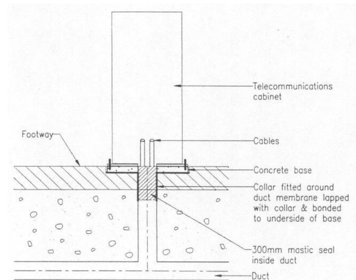
TYPICAL SURFACE DETAIL FOR ABOVE GROUND TERMINATION OF SERVICES WITHIN THE CONSULTATION ZONE (CROSS-SECTION)
