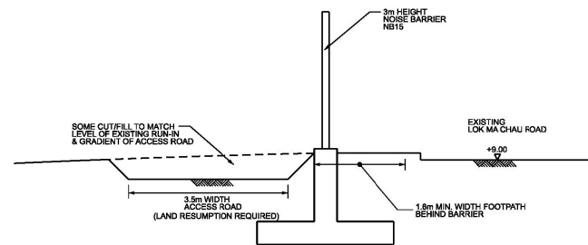
SECTION 2 - 2
