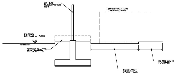
SECTION 1 - 1
