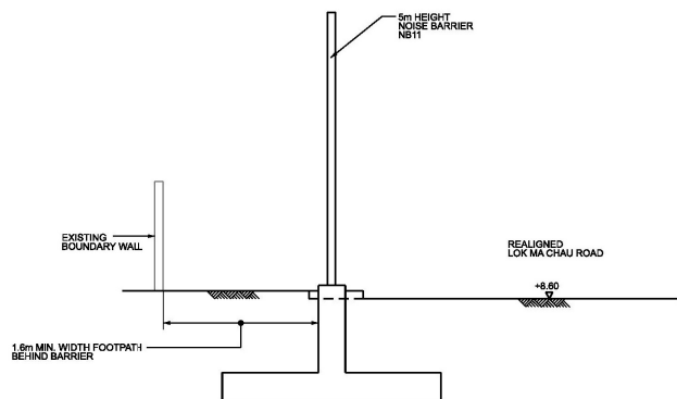
SECTION 3 - 3
