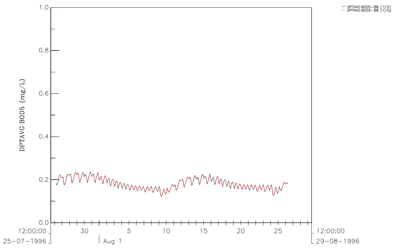
BOD5 Comparison between Scenario1 and Scenario2 at B2 (upper) and B8 (lower). Dry Season Figure 5C-24 DSD & ATKINS
