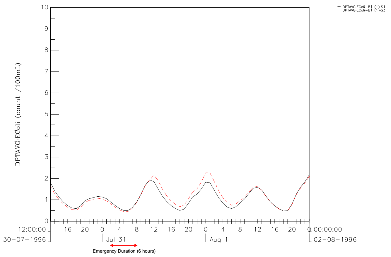
EColi Comparison between Scenario1 and Scenario3 at F1 (upper) and B1 (lower). Flood tide during Spring tide cycle. Dry Season Figure 5C-209 DSD & ATKINS
