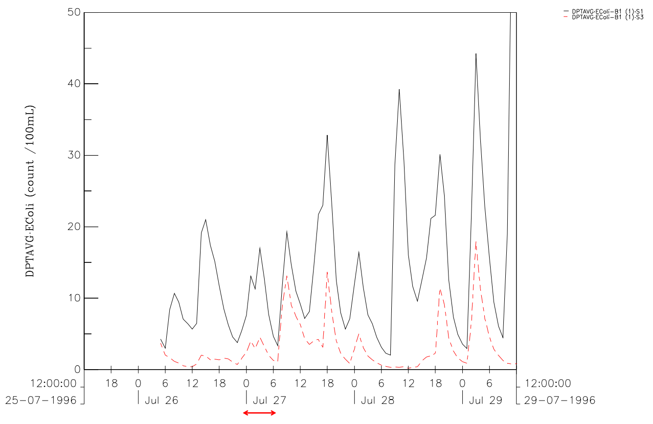
EColi Comparison between Scenario1 and Scenario3 at F1 (upper) and B1 (lower). Wet Season Figure 5C-143 DSD & ATKINS
