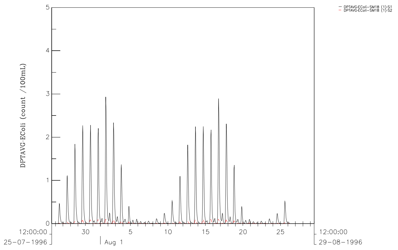
EColi Comparison between Scenario1 and Scenario2 at SM17 (upper) and SM18 (lower).
