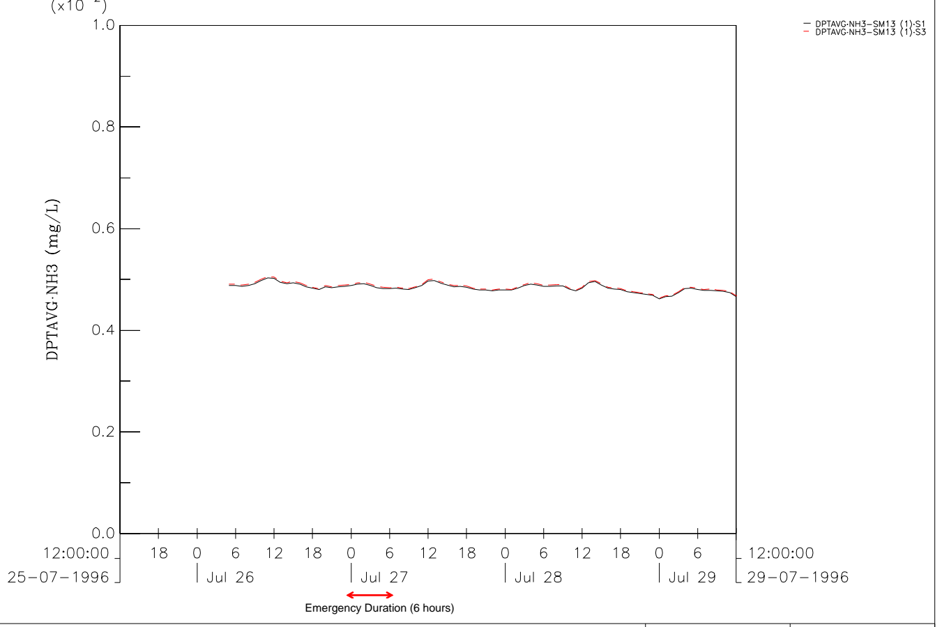
NH3 Comparison between Scenario1 and Scenario3 at SM12 (upper) and SM13 (lower). Wet Season Figure 5C-159 DSD & ATKINS
