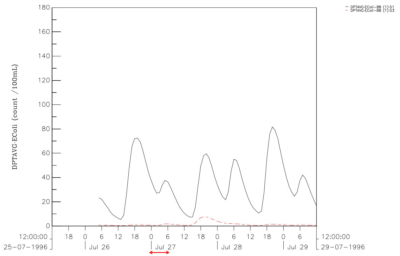
EColi Comparison between Scenario1 and Scenario3 at B2 (upper) and B8 (lower). Dry Season Figure 5C-134 DSD & ATKINS
