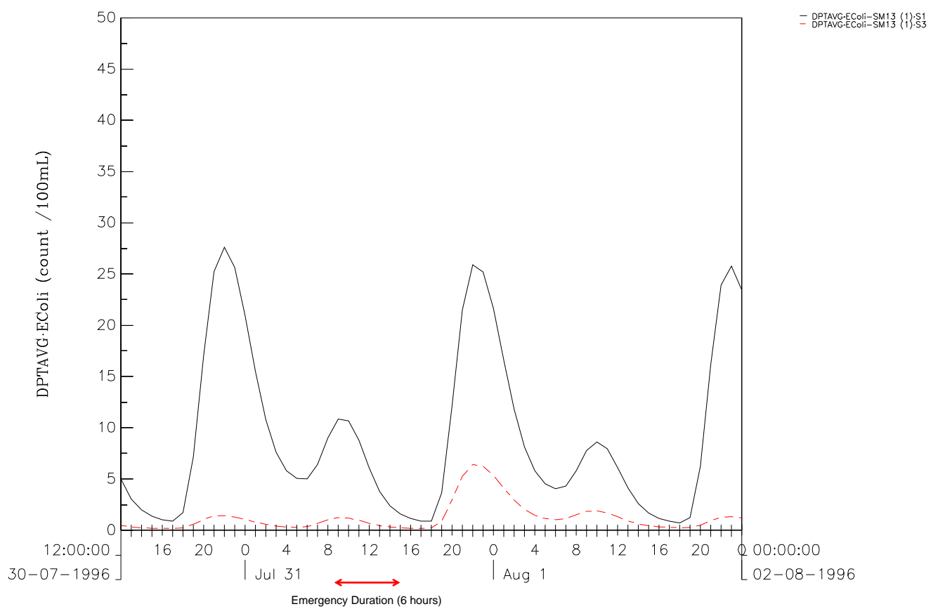
EColi Comparison between Scenario1 and Scenario3 at SM12 (upper) and SM13 (lower). Ebb tide during Spring tide cycle. Dry Season Figure 5C-219 DSD & ATKINS
