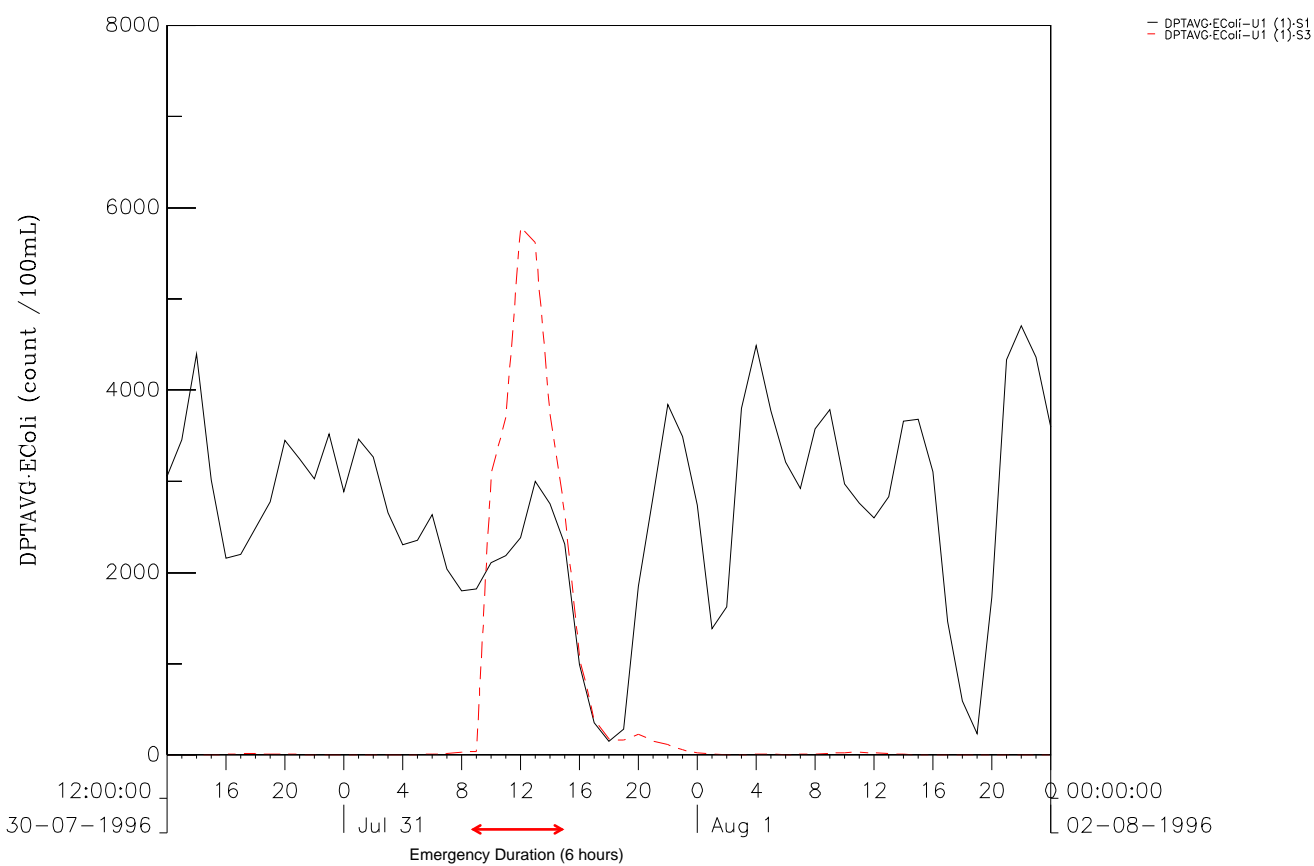
EColi Comparison between Scenario1 and Scenario3 at ST1 (upper) and U1 (lower). Ebb tide during Spring tide cycle. Wet Season Figure 5C-226 DSD & ATKINS
