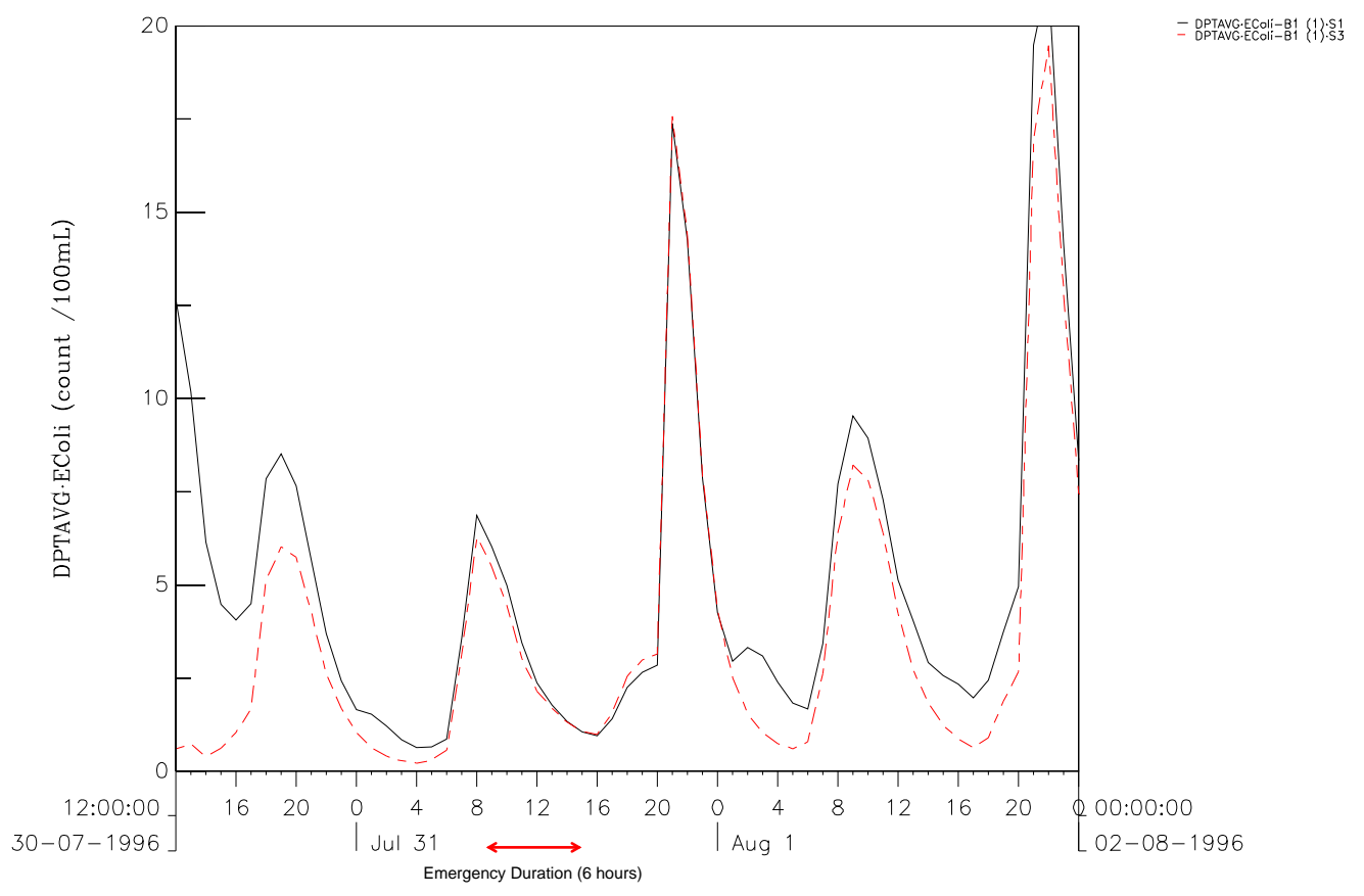
EColi Comparison between Scenario1 and Scenario3 at F1 (upper) and B1 (lower). Ebb tide during Spring tide cycle. Wet Season Figure 5C-227 DSD & ATKINS
