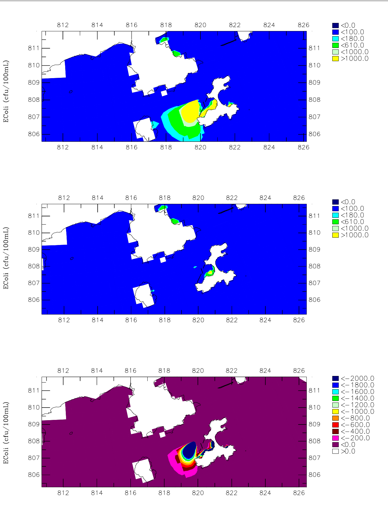
Simulated Depth Averaged EColi Distribution. Scenario 1 (upper), Scenario 2 (middle), Difference between Scenario 1 and Scenario 2 (lower).
