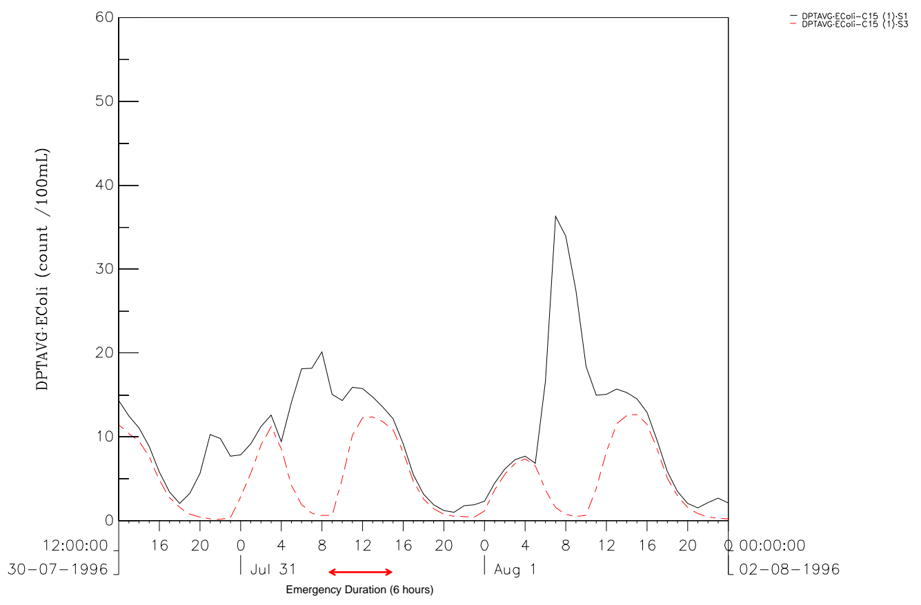
EColi Comparison between Scenario1 and Scenario3 at B9 (upper) and C15 (lower). Wet Season Figure 5C-229 DSD & ATKINS
