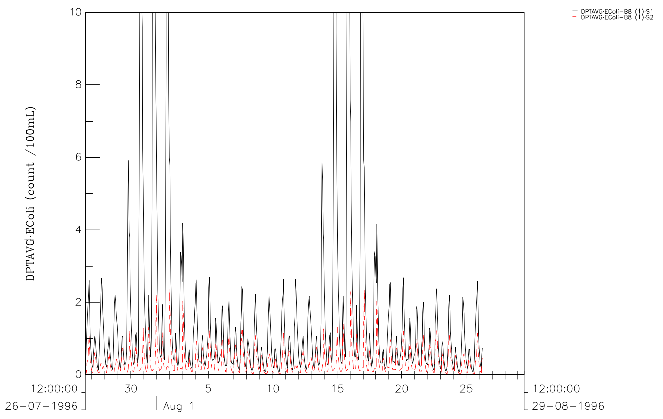
EColi Comparison between Scenario1 and Scenario2 at B2 (upper) and B8 (lower). wet season Figure 5C-69 DSD & ATKINS
