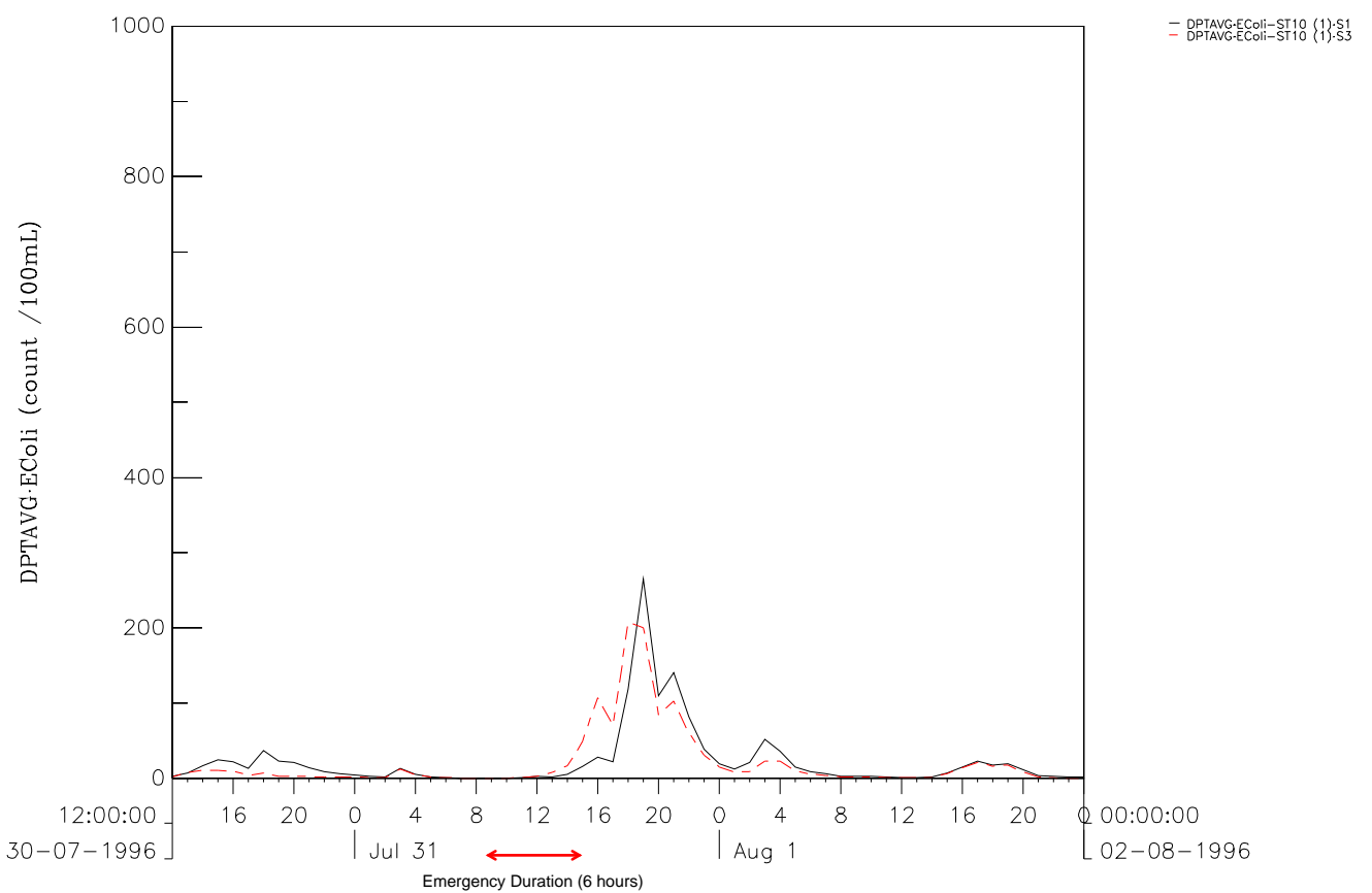
EColi Comparison between Scenario1 and Scenario3 at ST9 (upper) and ST10 (lower). Ebb tide during Spring tide cycle. Wet Season Figure 5C-230 DSD & ATKINS
