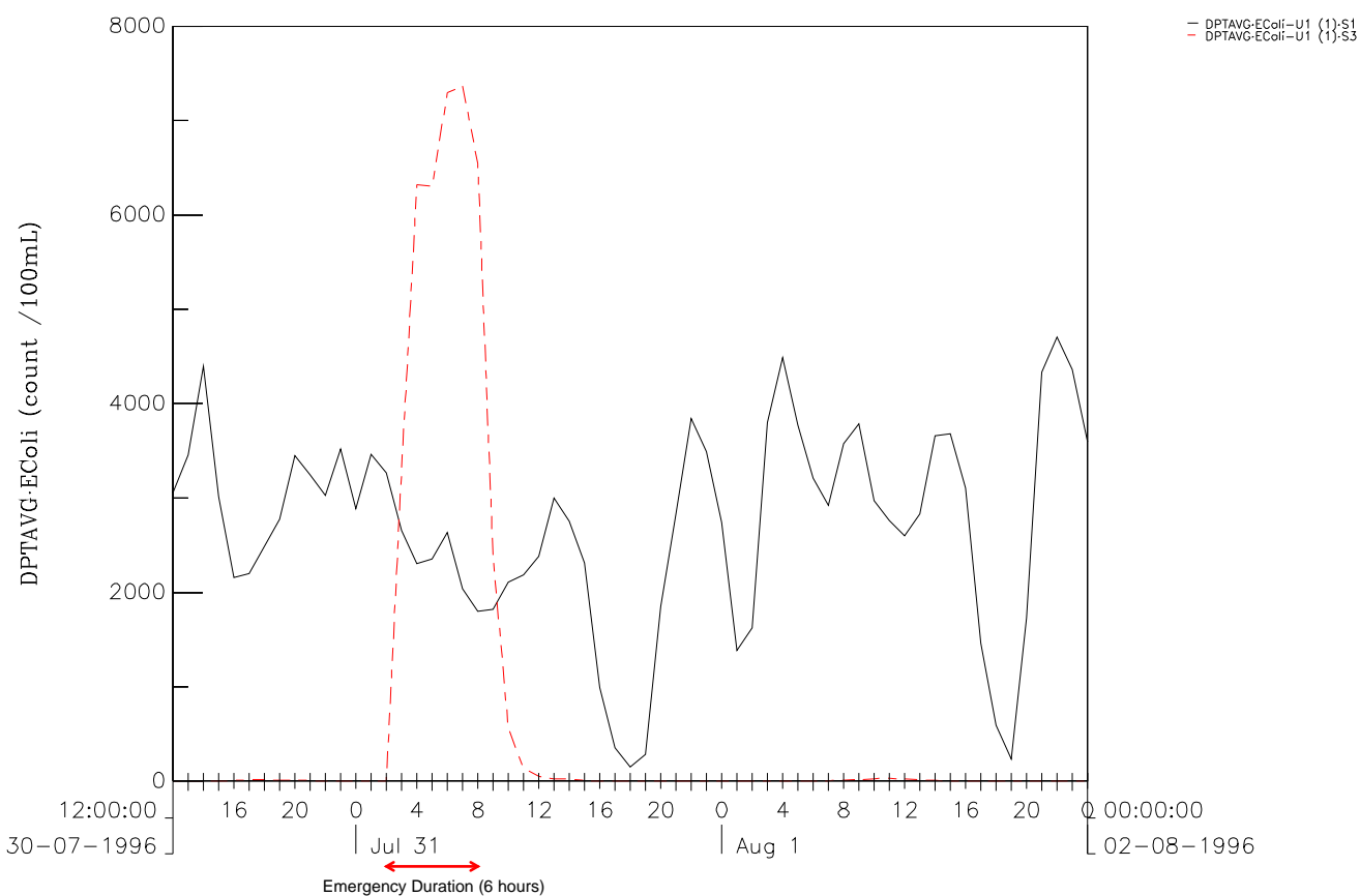
EColi Comparison between Scenario1 and Scenario3 at ST1 (upper) and U1 (lower). Flood tide during Spring tide cycle. Wet Season Figure 5C-214 DSD & ATKINS
