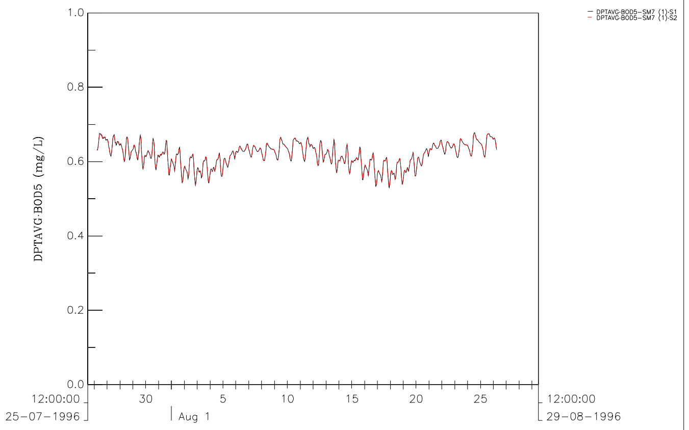
BOD5 Comparison between Scenario1 and Scenario2 at SM6 (upper) and SM7 (lower). wet season Figure 5C-30 DSD & ATKINS
