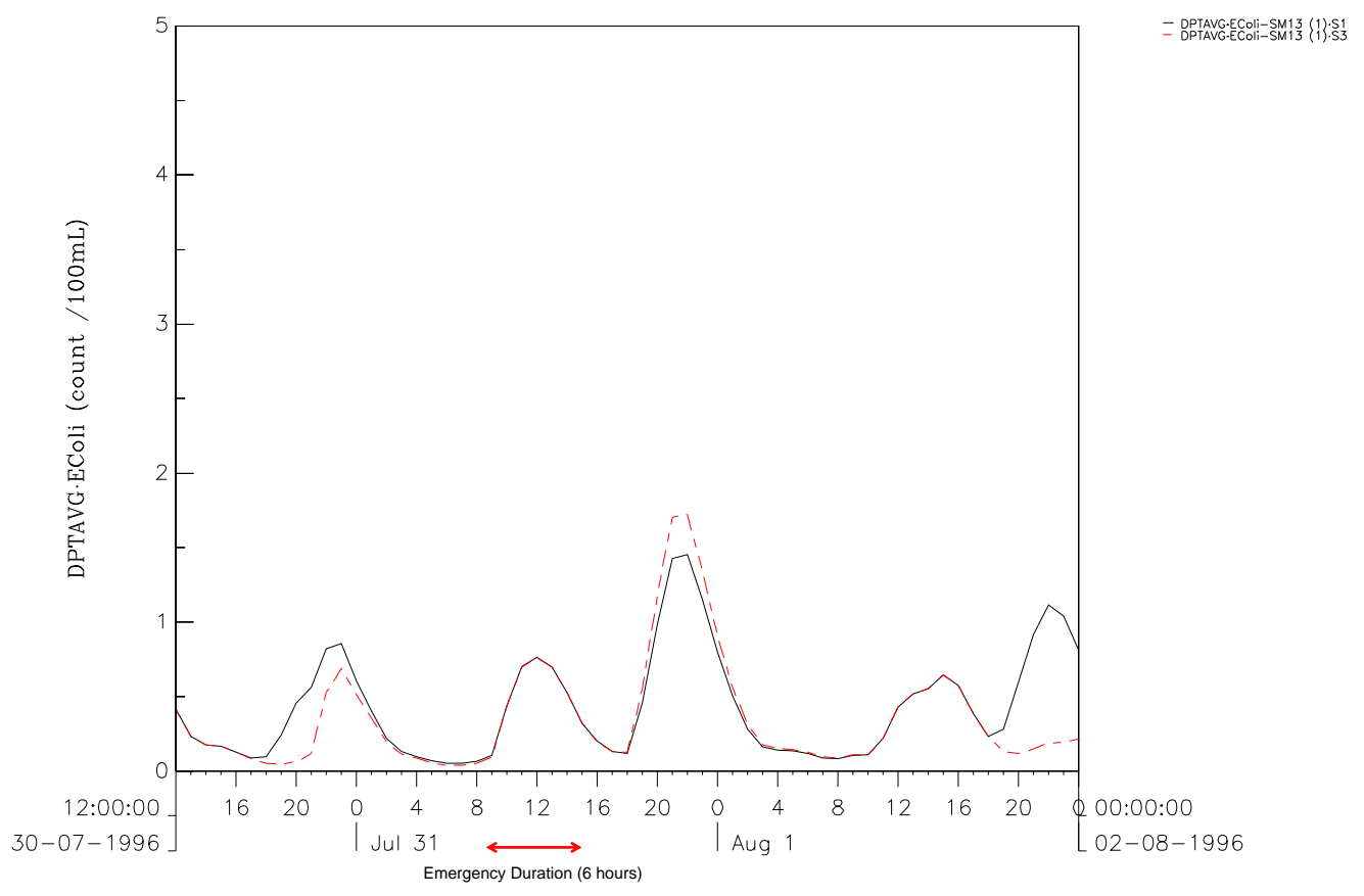
EColi Comparison between Scenario1 and Scenario3 at SM12 (upper) and SM13 (lower). Ebb tide during Spring tide cycle. Wet Season Figure 5C-225 DSD & ATKINS
