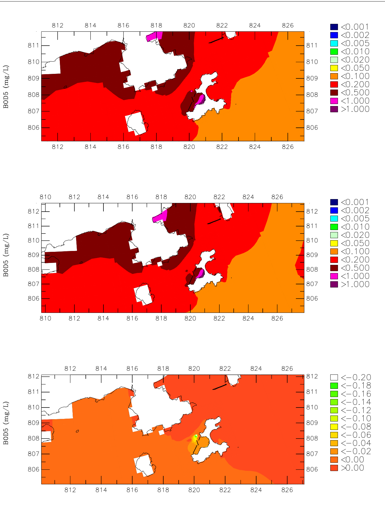
Simulated Depth Averaged BOD5 Distribution. Scenario 1 (upper), Scenario 2 (middle), Difference between Scenario 1 and Scenario 2 (lower).
