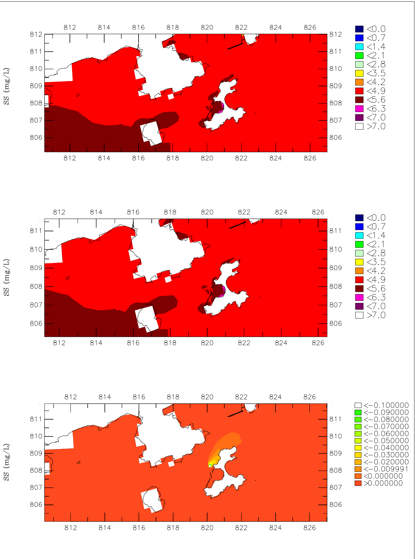
Simulated Depth Averaged SS Distribution. Scenario 1 (upper), Scenario 2 (middle), Difference between Scenario 1 and Scenario 2 (lower).
