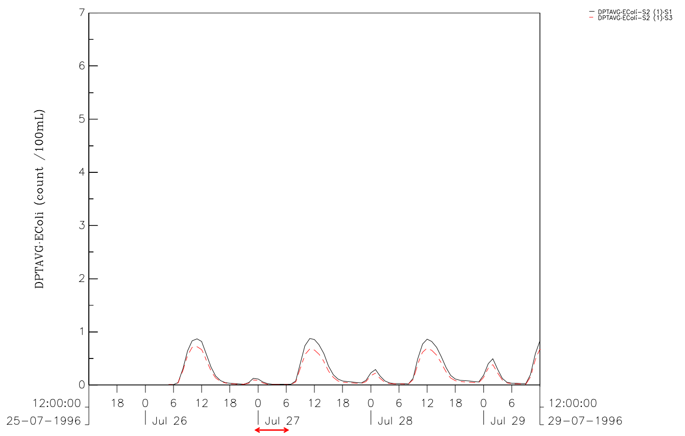
EColi Comparison between Scenario1 and Scenario3 at C4 (upper) and S2 (lower). Dry Season Figure 5C-127 DSD & ATKINS
