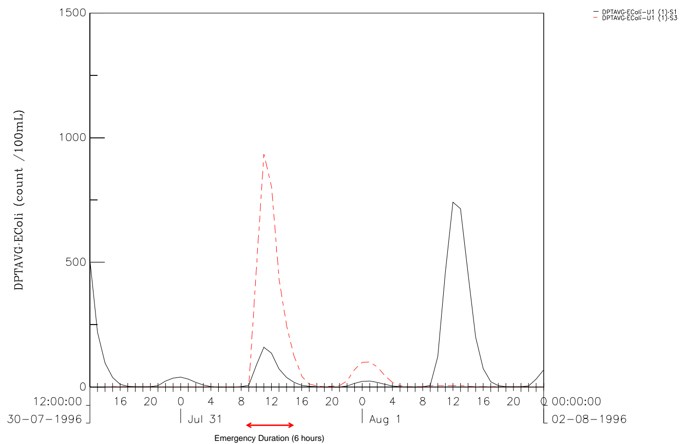
EColi Comparison between Scenario1 and Scenario3 at ST1 (upper) and U1 (lower). Ebb tide during Spring tide cycle. Dry Season Figure 5C-220 DSD & ATKINS
