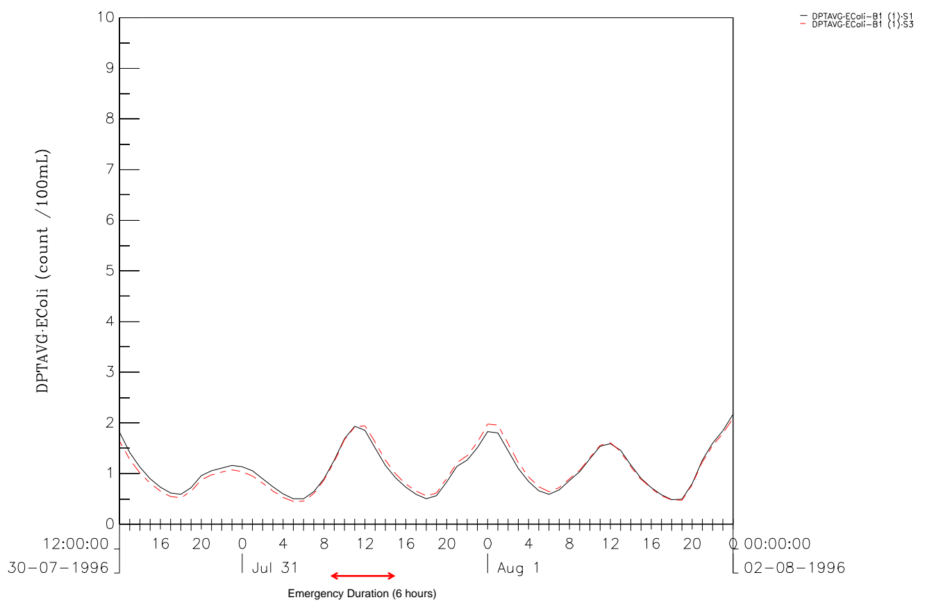
EColi Comparison between Scenario1 and Scenario3 at F1 (upper) and B1 (lower). Ebb tide during Spring tide cycle. Dry Season Figure 5C-221 DSD & ATKINS
