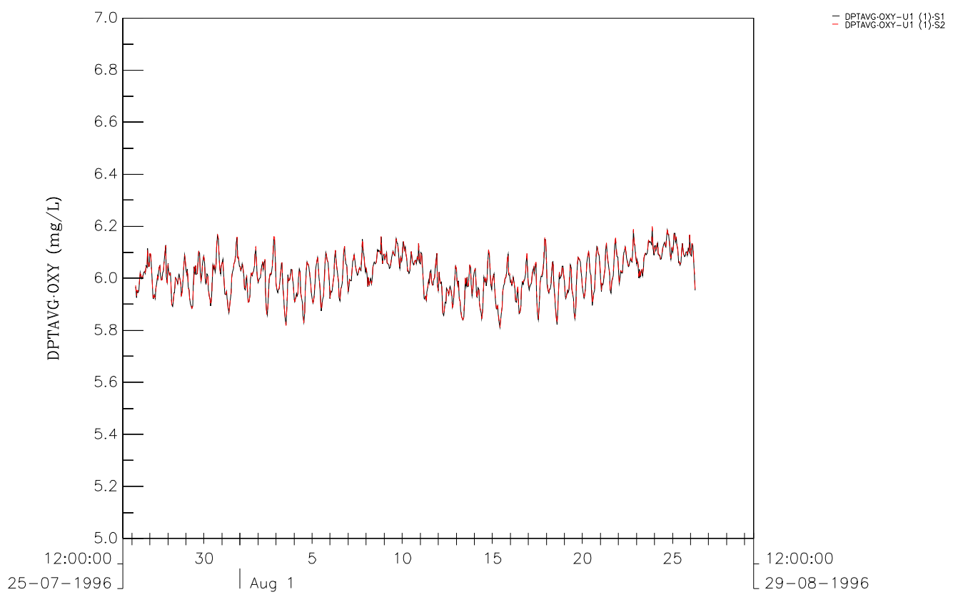
OXY Comparison between Scenario1 and Scenario2 at ST1 (upper) and U1 (lower). wet season Figure 5C-49 DSD & ATKINS
