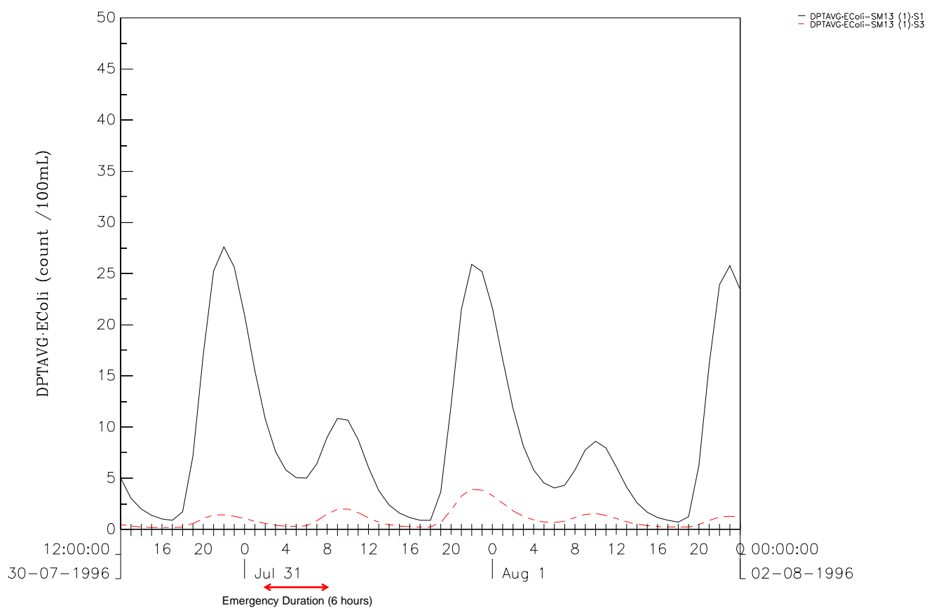
EColi Comparison between Scenario1 and Scenario3 at SM12 (upper) and SM13 (lower). Flood tide during Spring tide cycle. Dry Season Figure 5C-207 DSD & ATKINS
