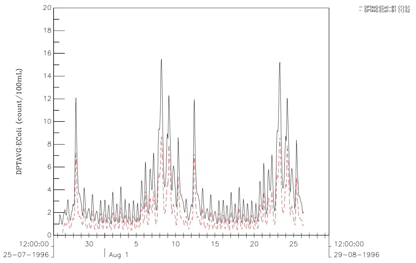
EColi Comparison between Scenario1 and Scenario2 at F1 (upper) and B1 (lower). Dry Season Figure 5C-59 DSD & ATKINS
