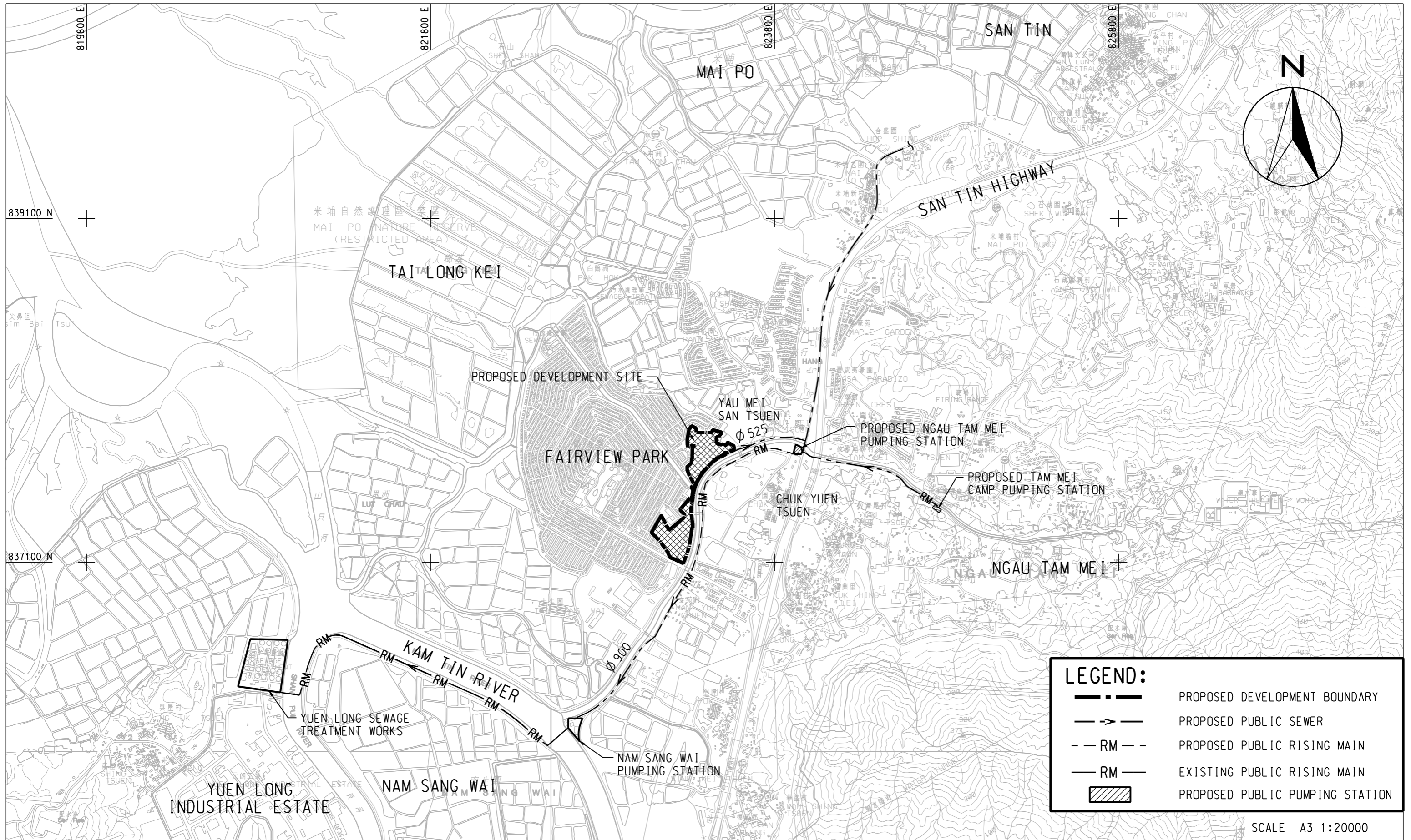
Figure: 6 - 2 Title: PROPOSED NGAU TAM MEI TRUNK SEWERAGE
