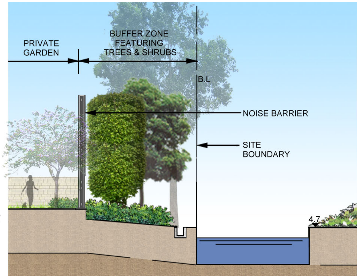
TYPICAL SECTION
