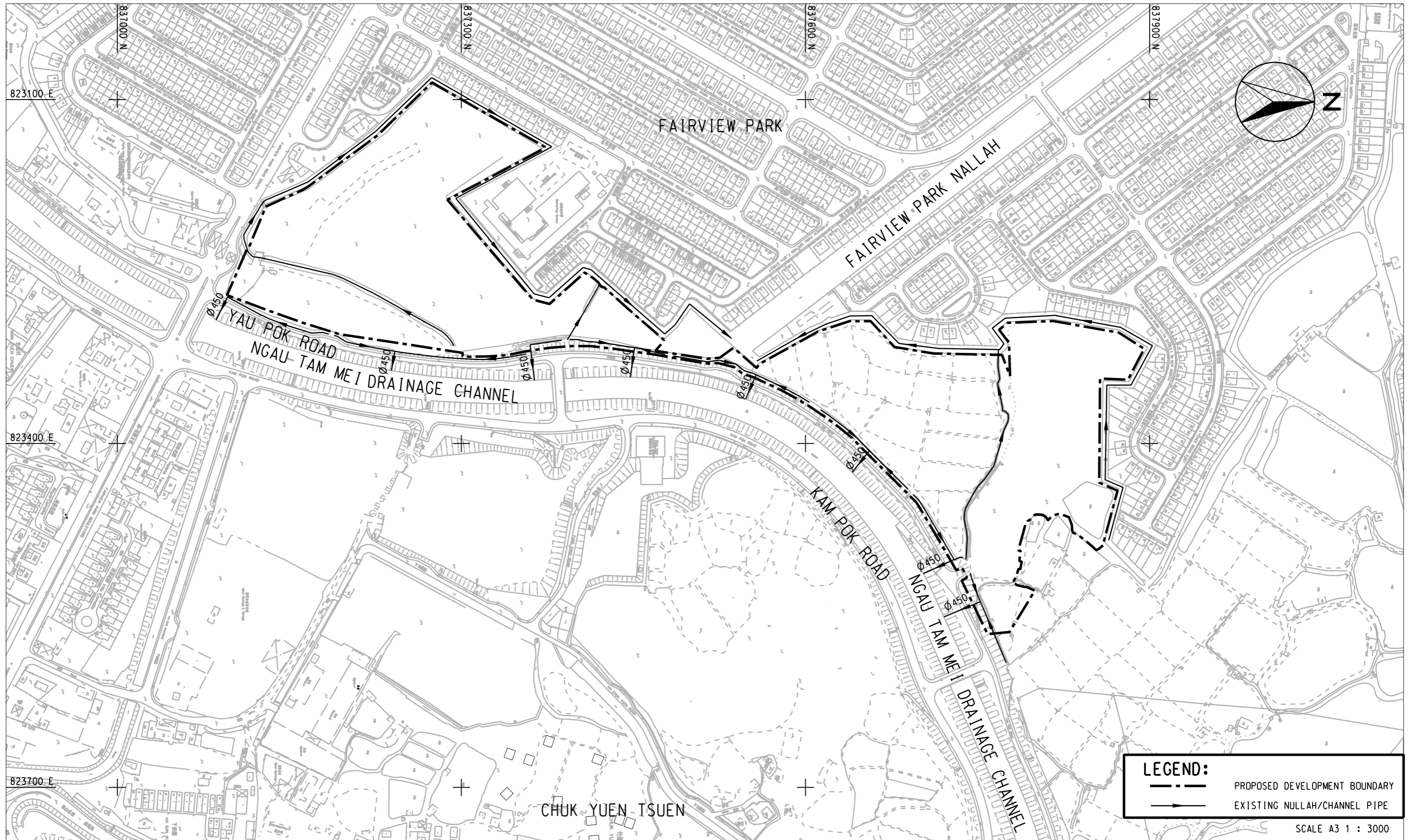
Figure: 5-3 Title: EXISTING DRAINAGE CONDITION
