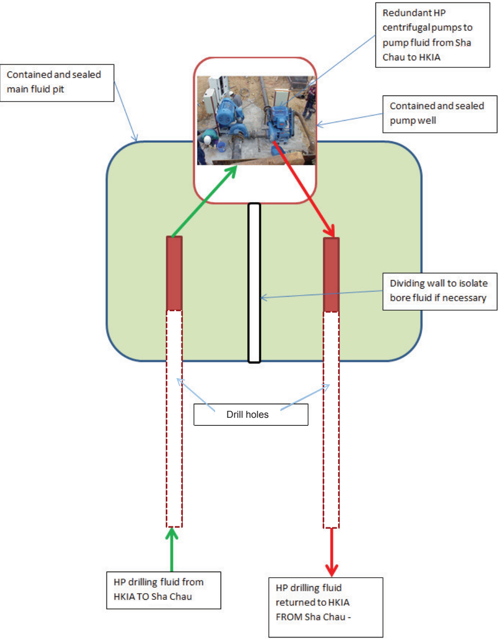
Figure B. Illustration of HDD drilling fluid recirculation system at Sha Chau
