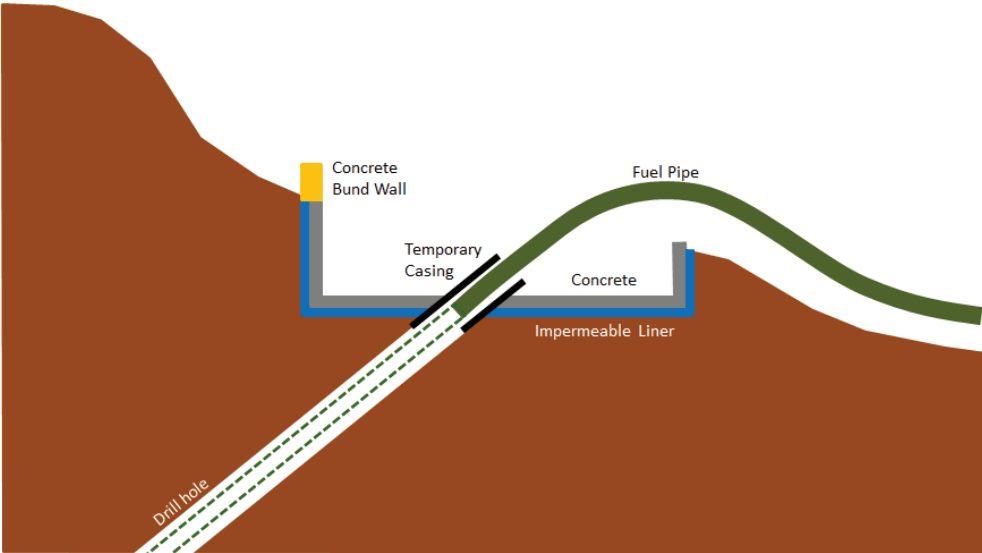
Figure A. Illustration of HDD containment pit at Sha Chau
