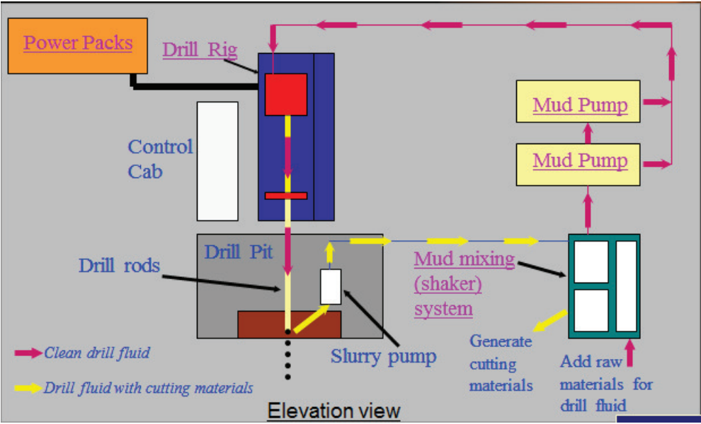
Figure C. Illustration of HDD process (Airport island side)
