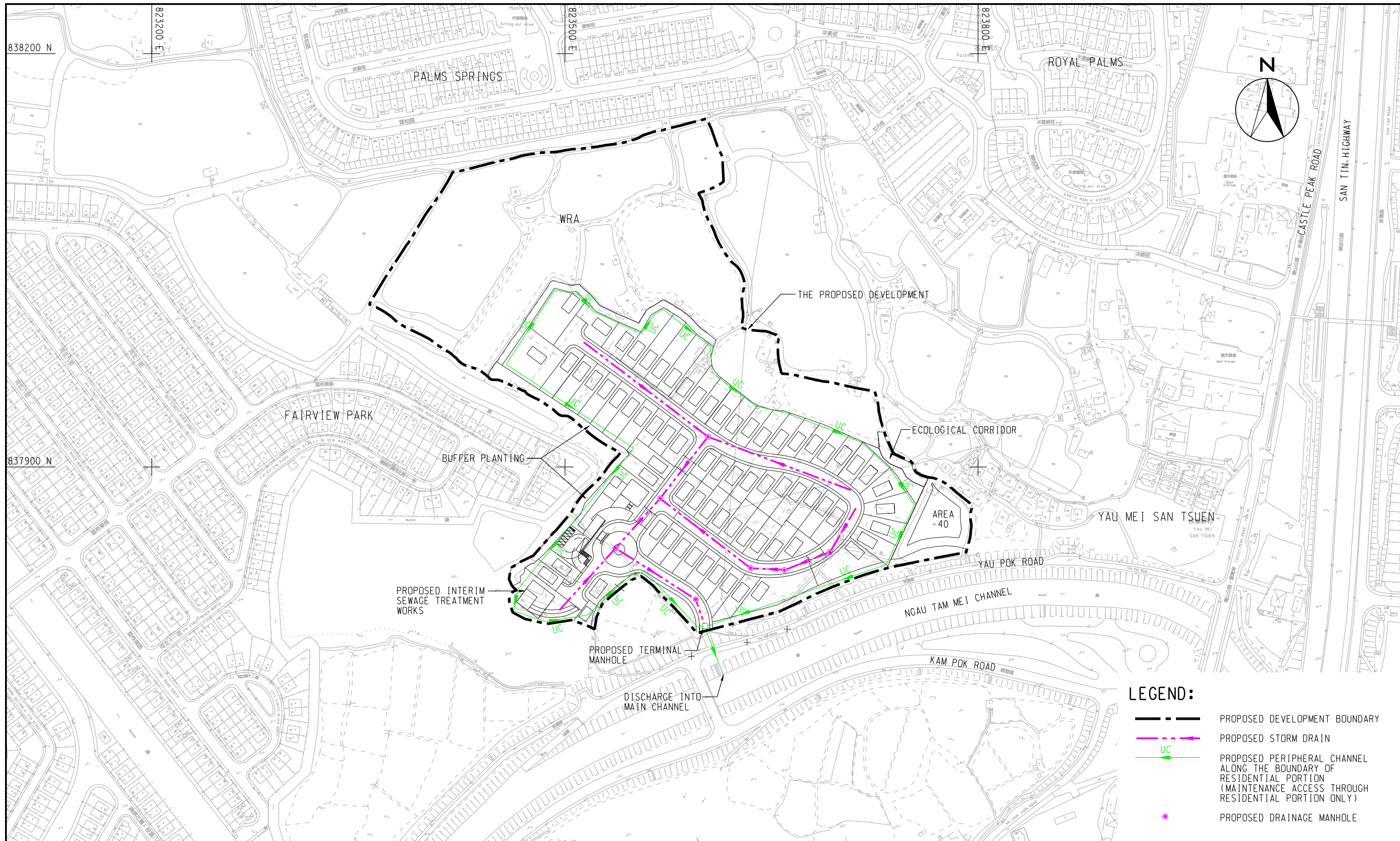
Figure: 5-3 Title: PROPOSED DRAINAGE SYSTEM
