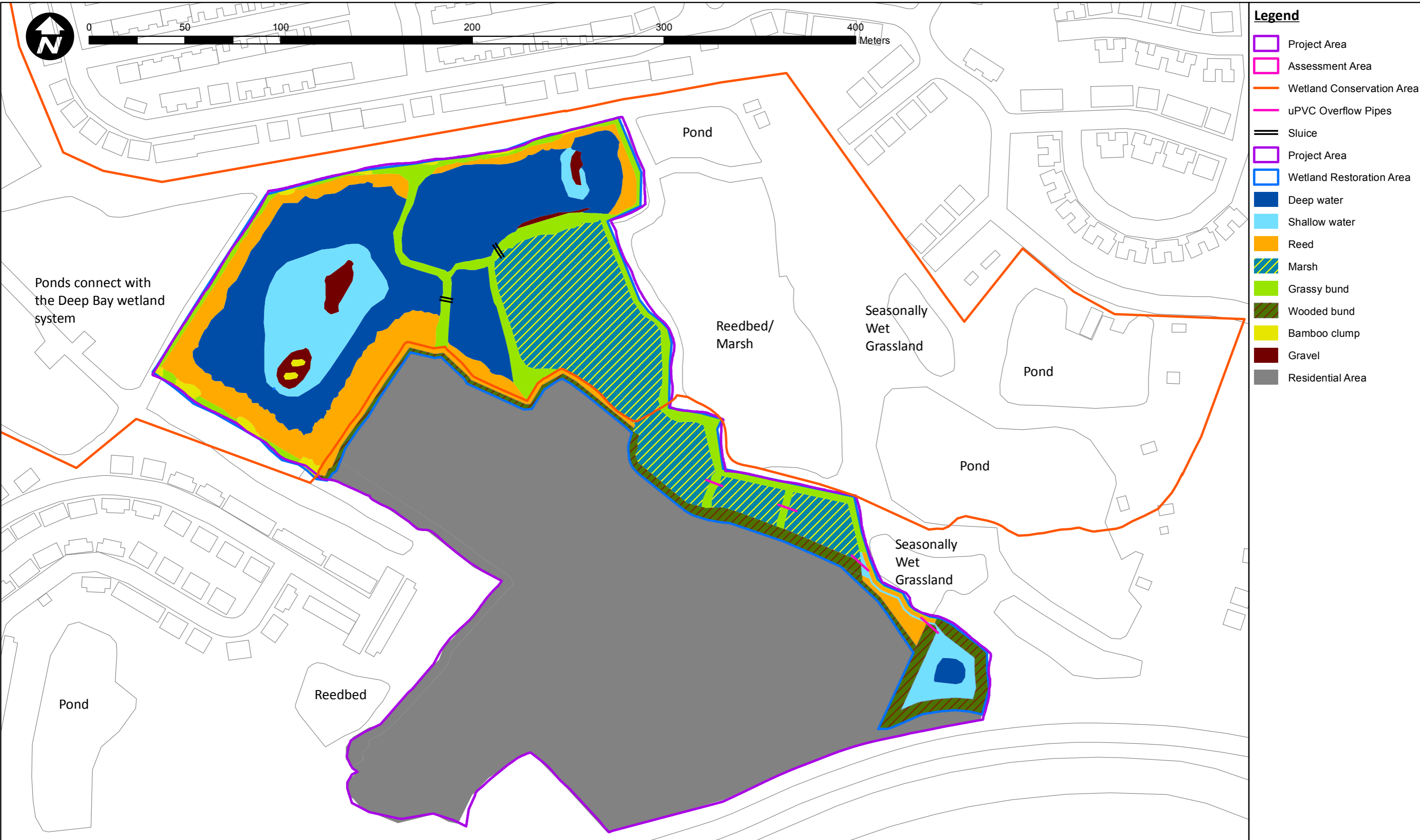
Figure: 8-5 ENVIRON Title: Proposed Layout of Wetland Restoration Plan Drawn by: JH Checked by: TC Project: Comprehensive Development and Wetland Protection near Yau Mei San Tsuen Rev: 4.3 Date: OCT 2014
