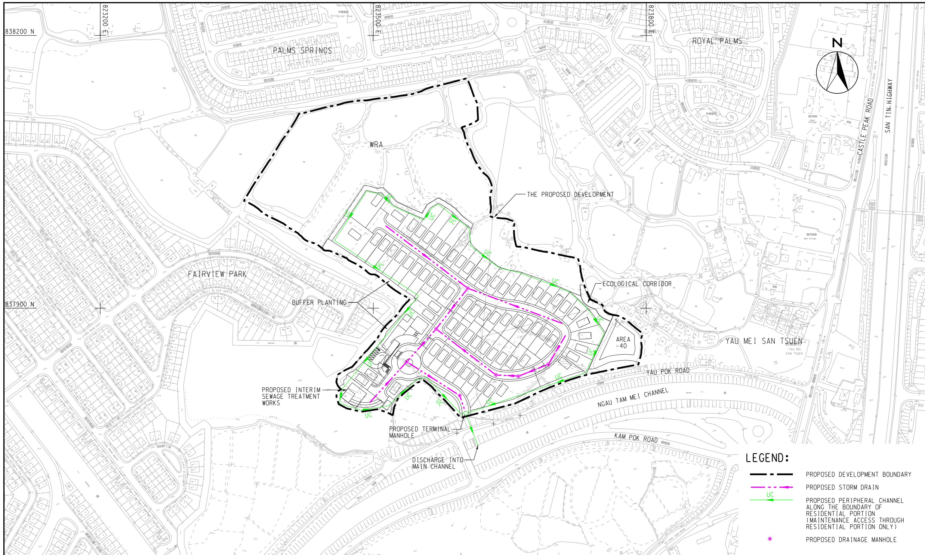
Figure: 6-3 Title: PROPOSED DRAINAGE SYSTEM
