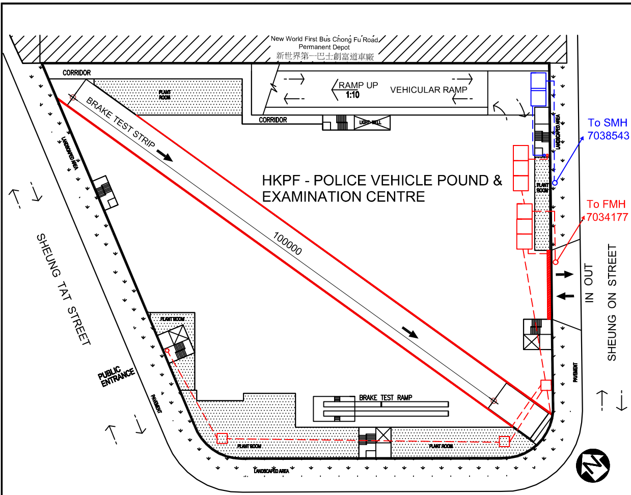
LEVEL 1 (+5.00) FLOOR PLAN
