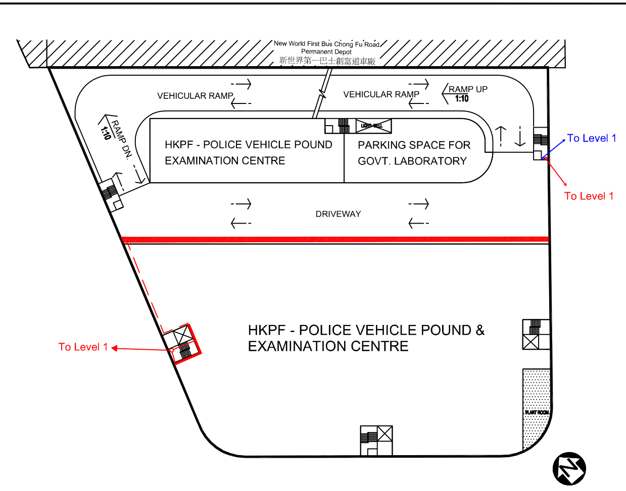
LEVEL 2 (+13.00) FLOOR PLAN
