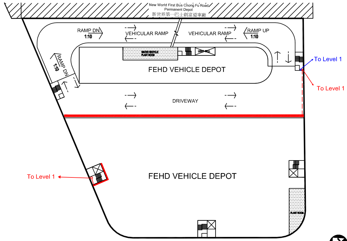
LEVEL 4 (+26.90) FLOOR PLAN
