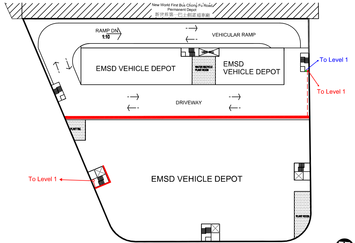
LEVEL 5 (+33.10) FLOOR PLAN
