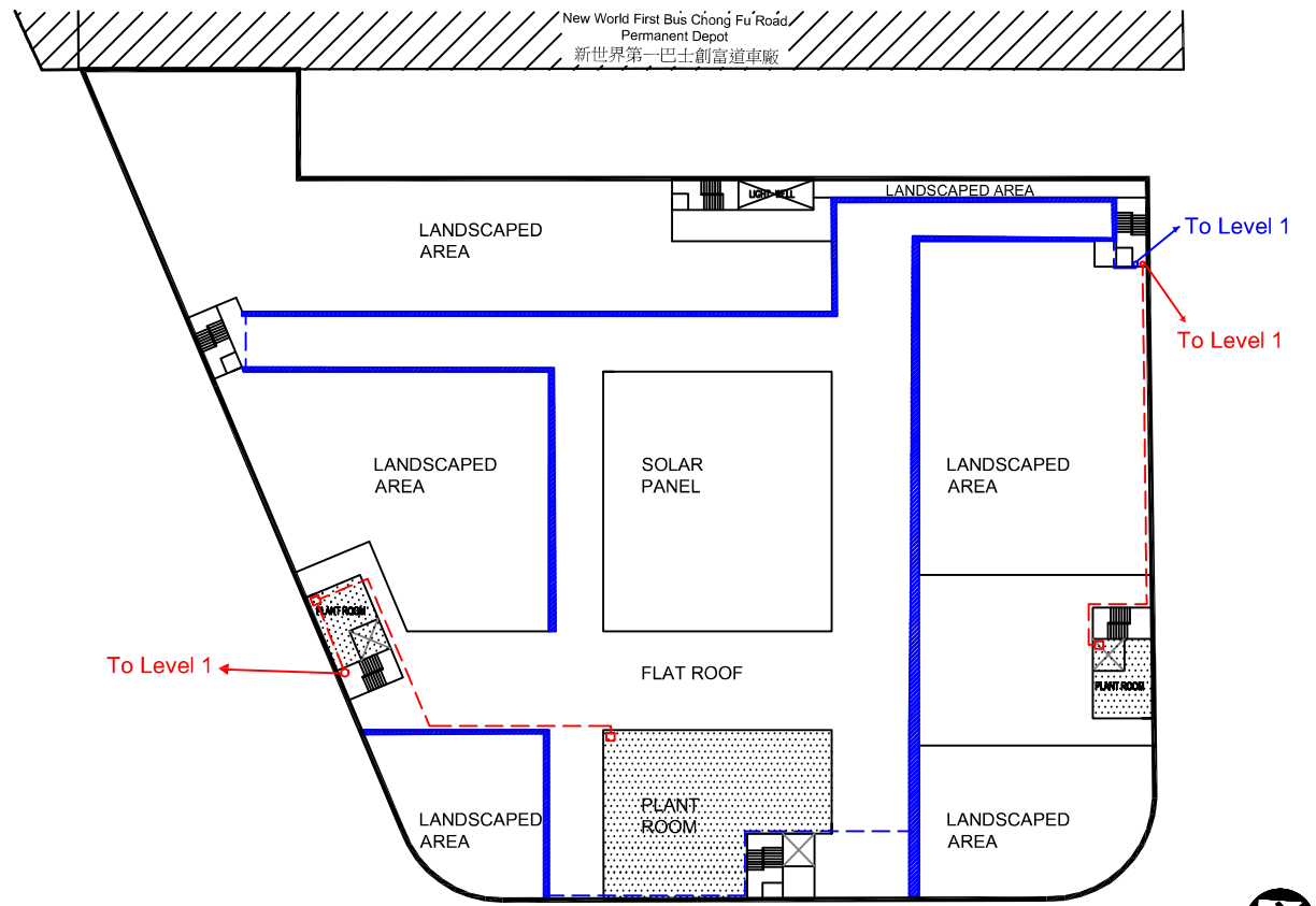
ROOF PLAN (+45.00)
