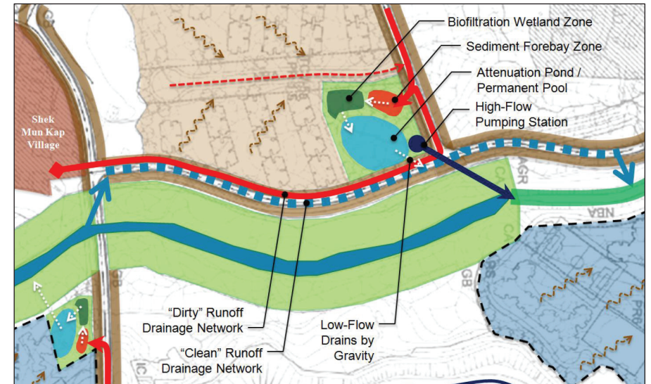
Conceptual Layout of Attenuation and Treatment Ponds
