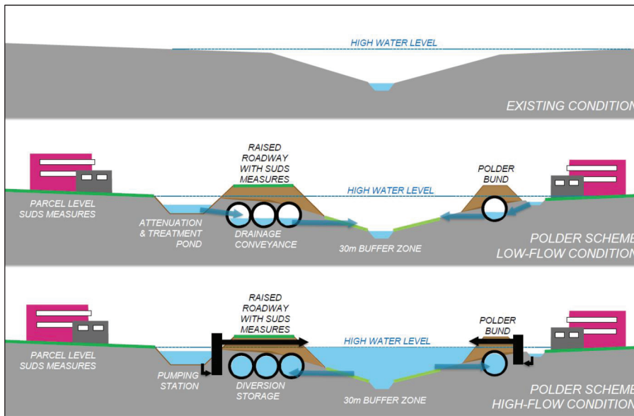
Proposed Drainage Conveyance and Diversion Storage under the Polder Scheme
