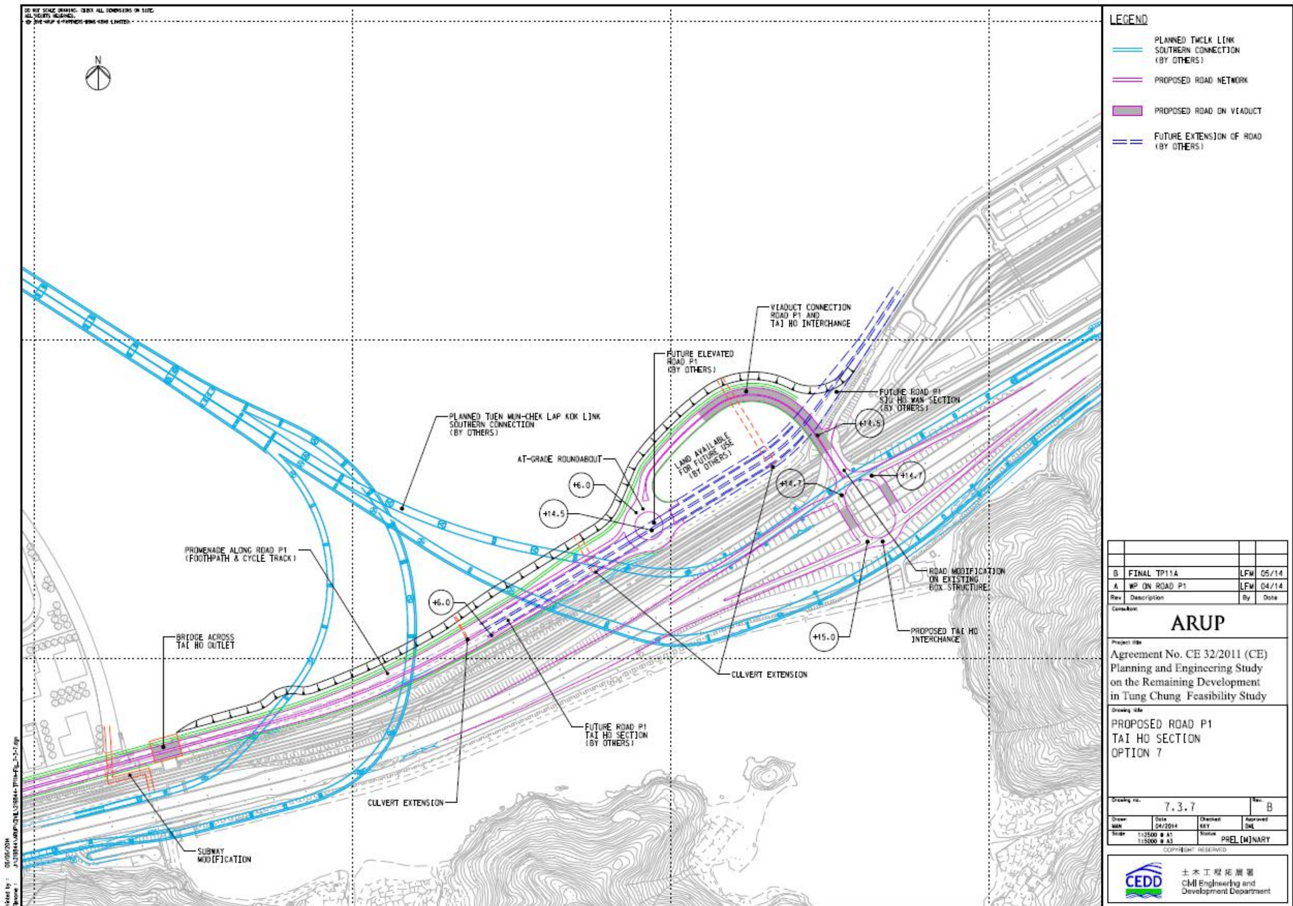
Proposed Road P1 (Tung Chung – Tai Ho Section) – Option F
