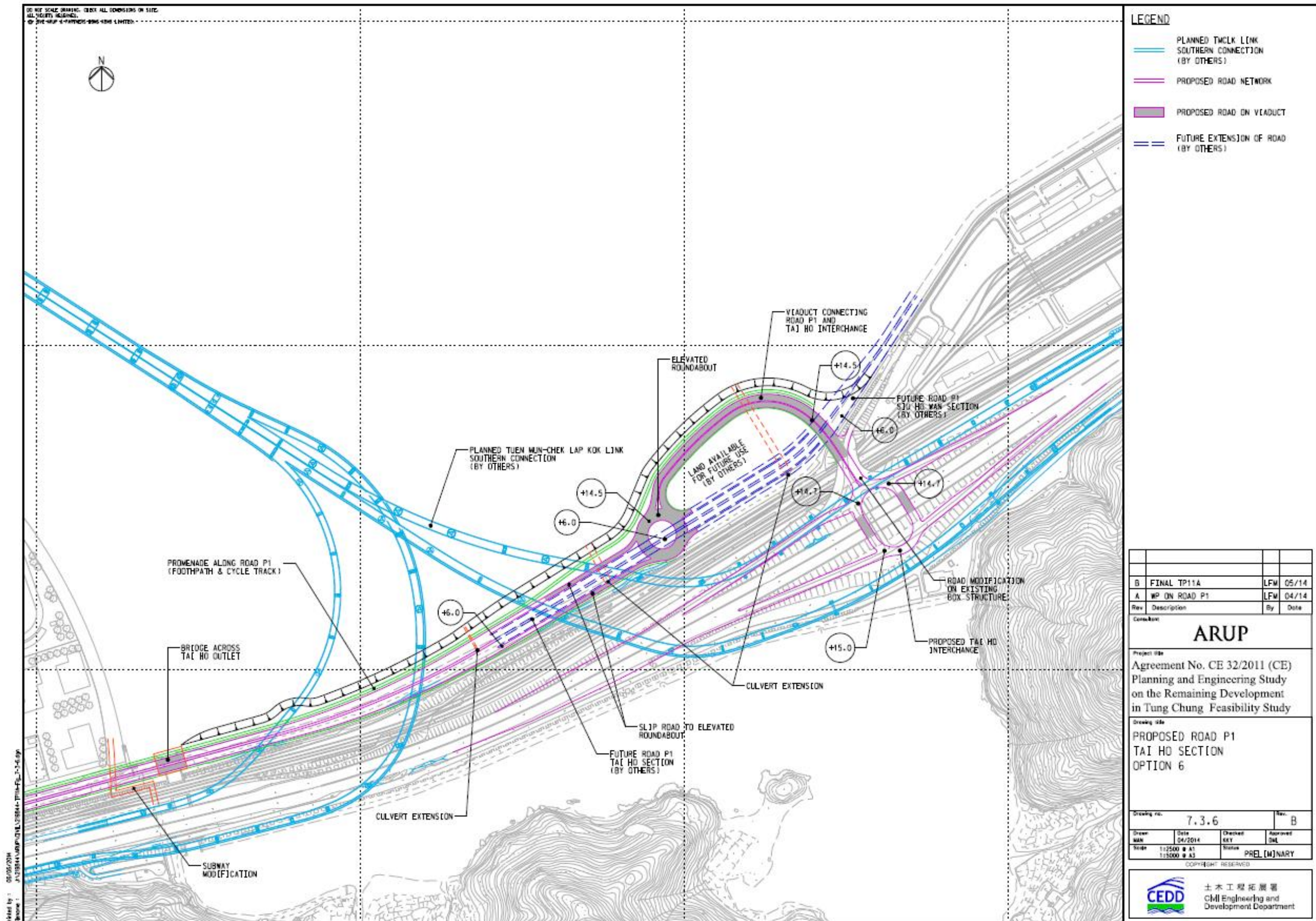
Proposed Road P1 (Tung Chung – Tai Ho Section) – Option E
