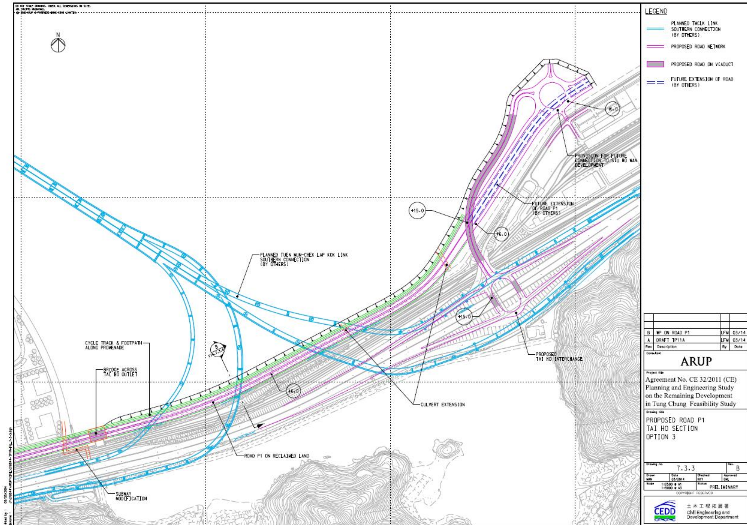
Proposed Road P1 (Tung Chung – Tai Ho Section) – Option B
