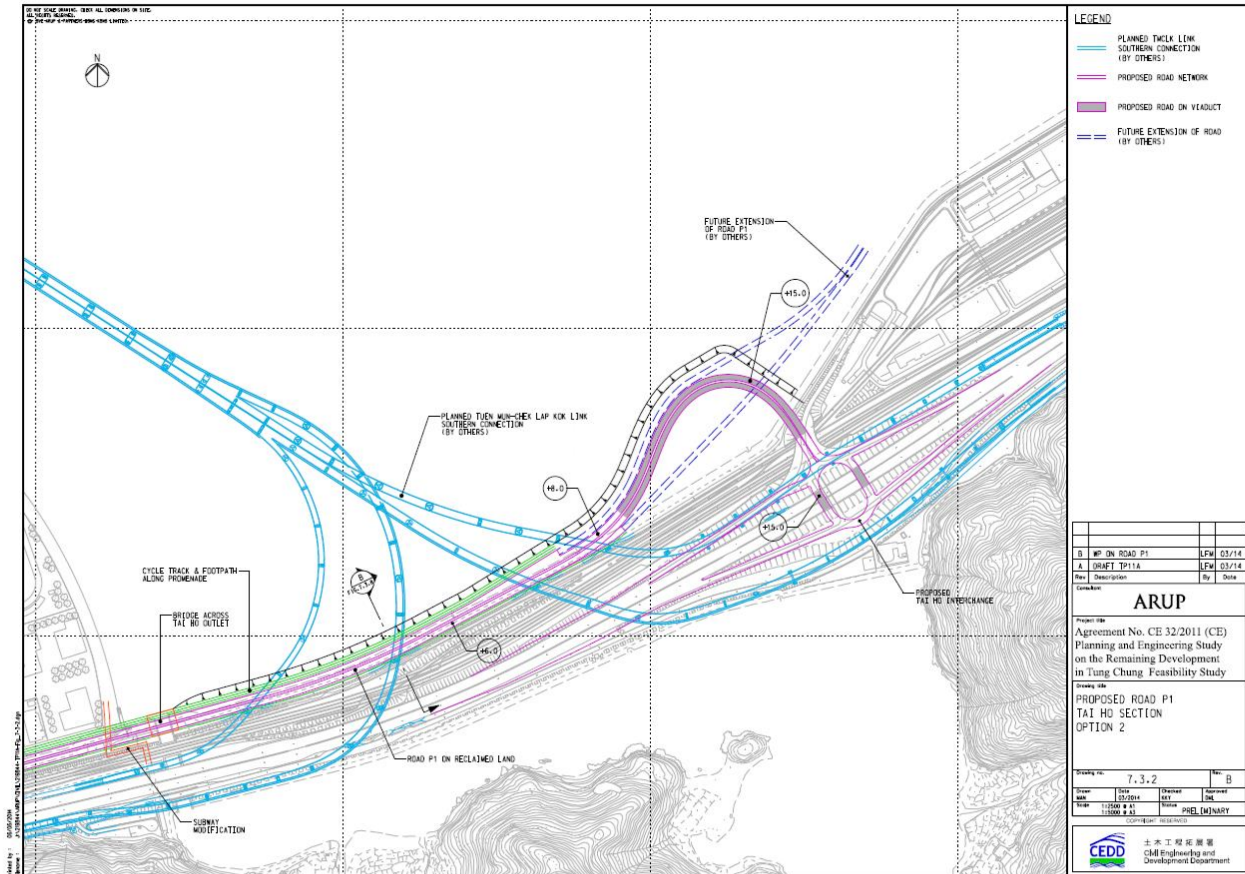
Proposed Road P1 (Tung Chung – Tai Ho Section) – Option A
