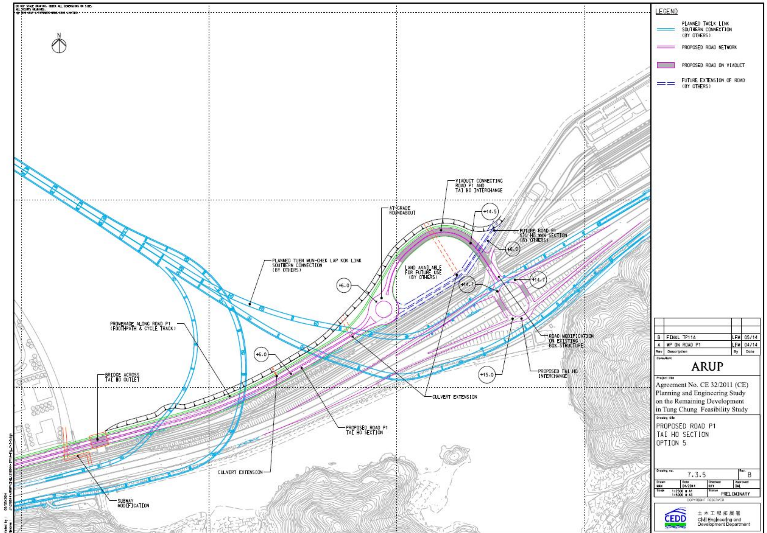
Proposed Road P1 (Tung Chung – Tai Ho Section) – Option D
