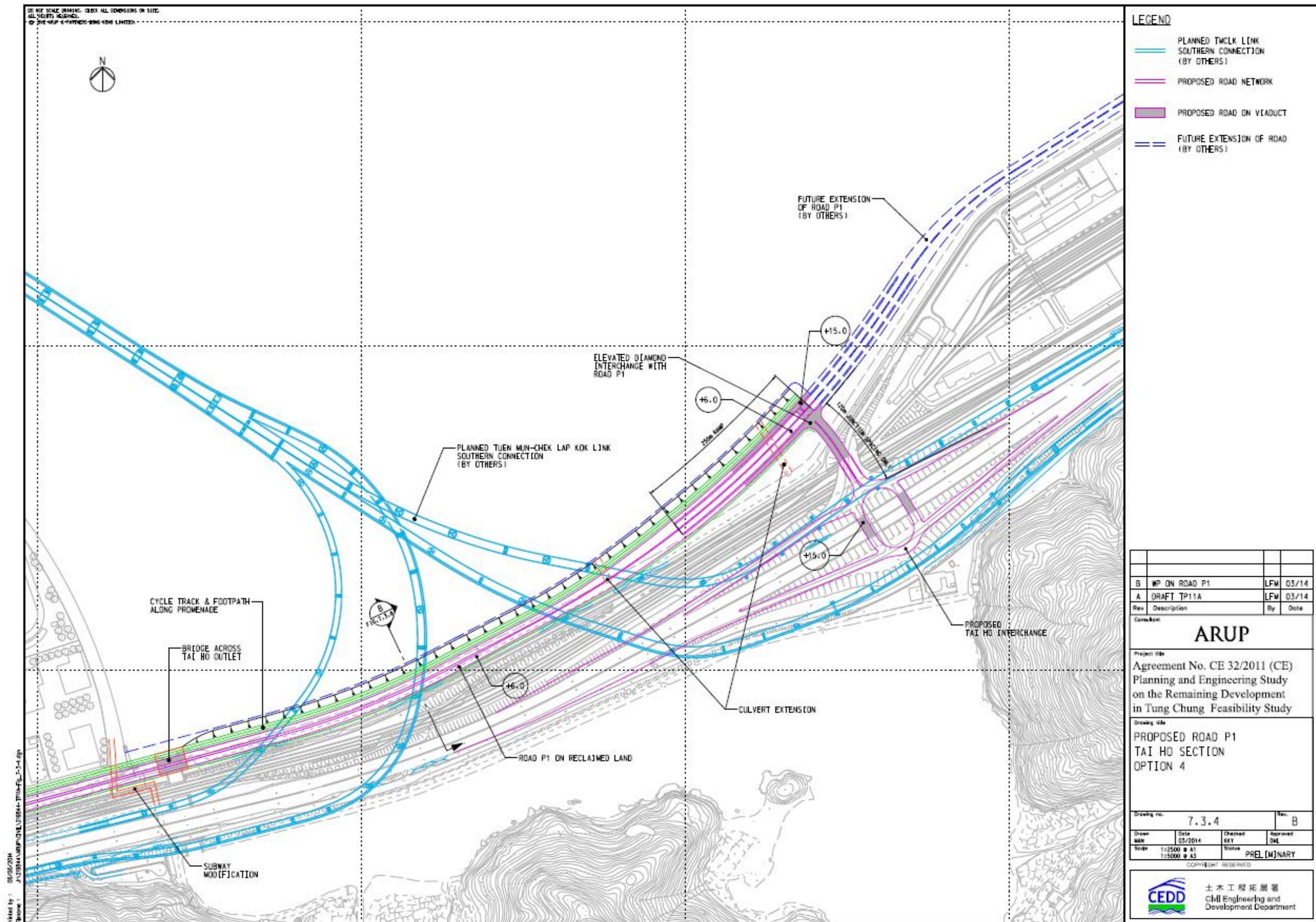
Proposed Road P1 (Tung Chung – Tai Ho Section) – Option C
