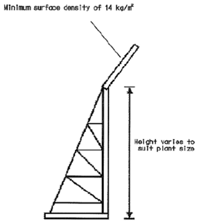
Typical Temporary Noise Barrier for Mobile Plant (~3-5m tall)
