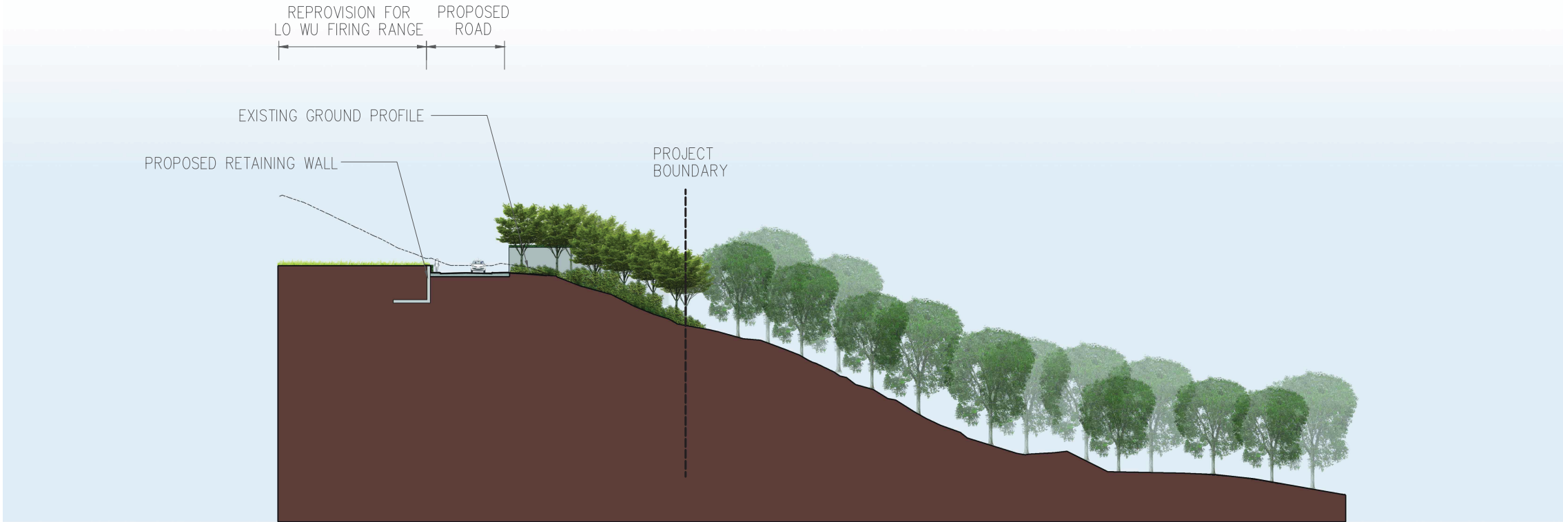
Section MMDP-6
