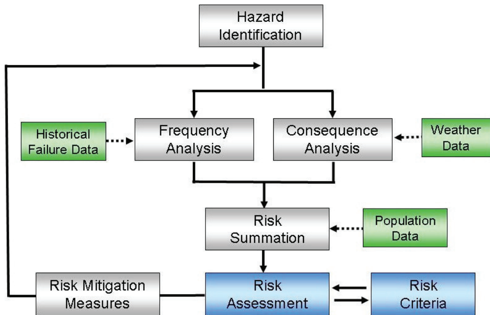
Figure 11-2: QRA Flow Chart
