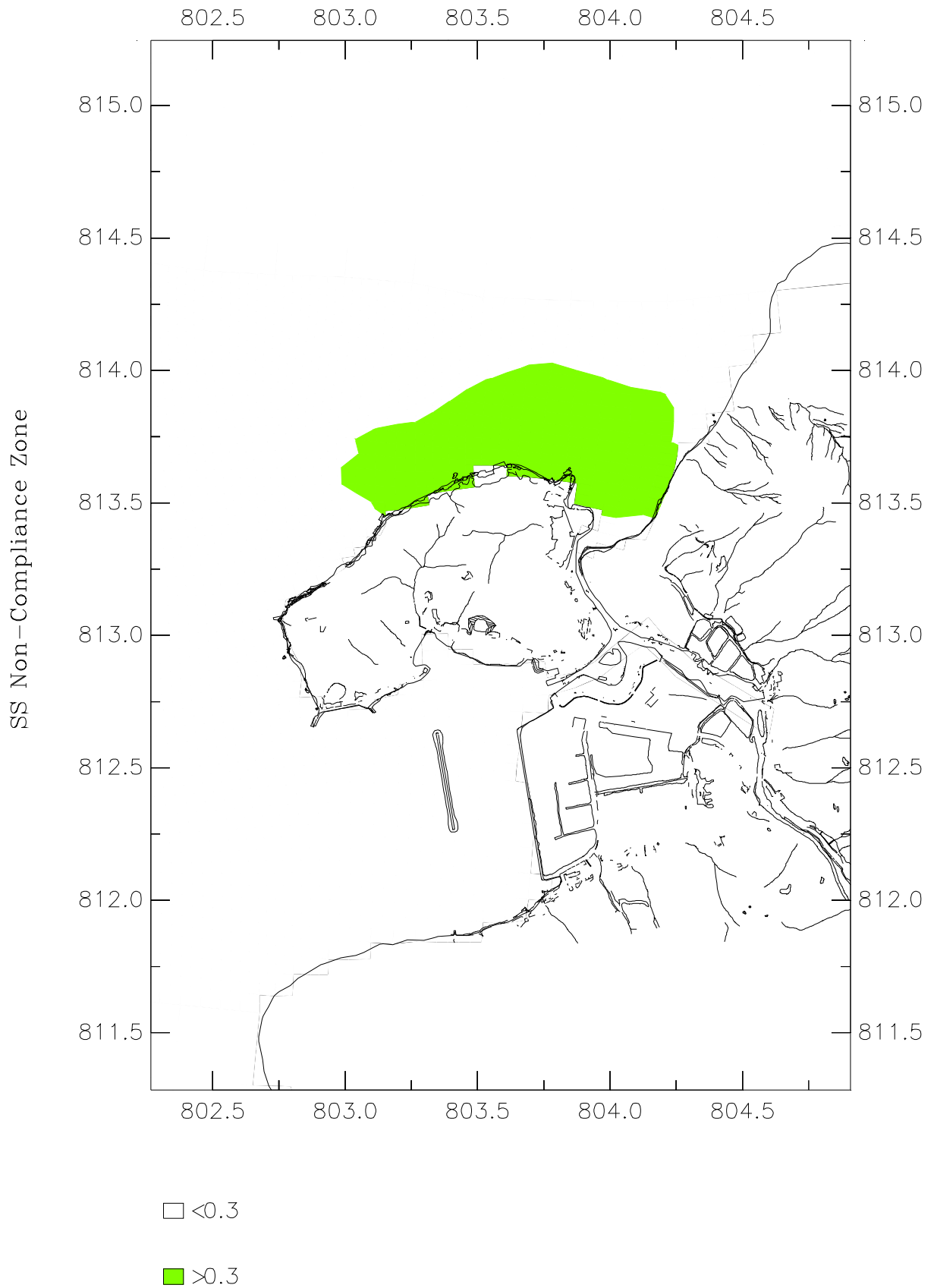
Suspended Solid Non-Compliance Zone Distribution Worst Case – Bottom Layer
