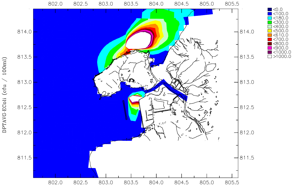
Simulated Depth Averaged EColi Normal Operation (Upper) and Maximum Concentration (Lower) occurred at 02:00 Jul 27 during Emergency Discharge.
