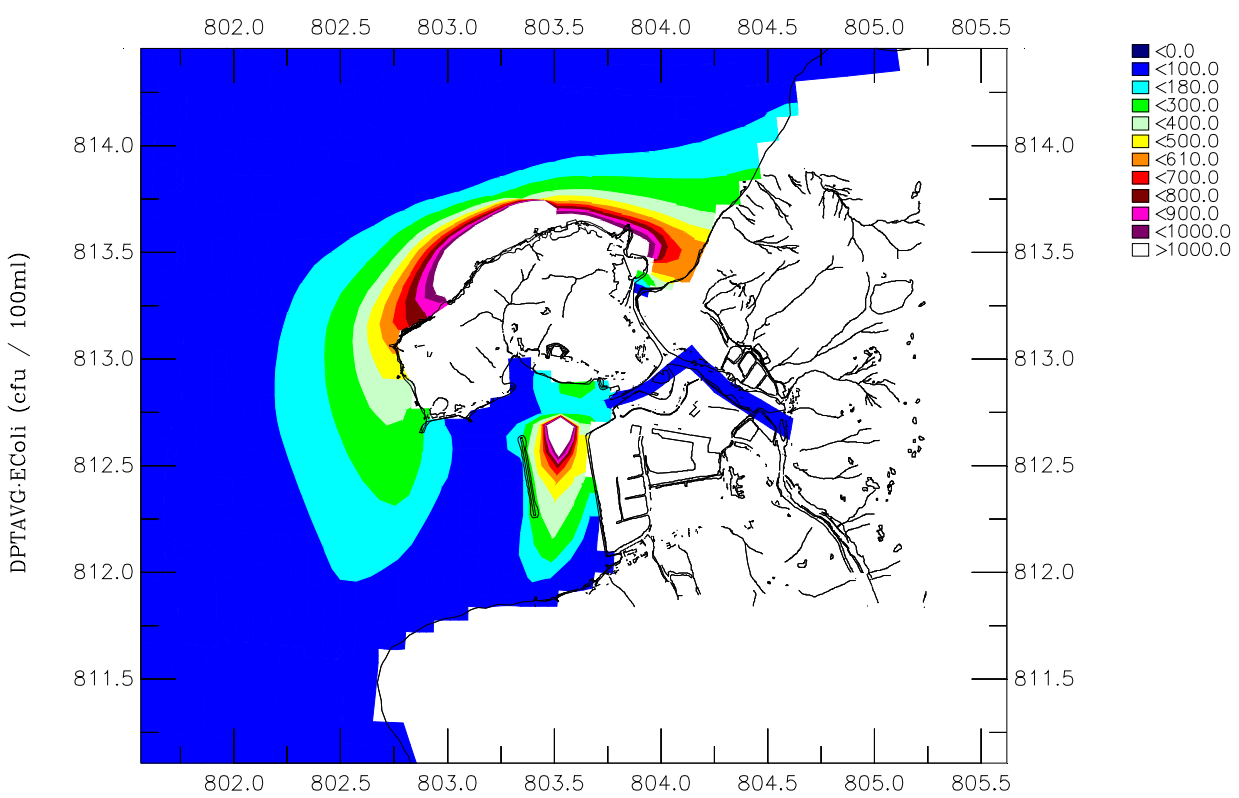
Simulated Depth Averaged EColi Normal Operation (Upper) and Maximum Concentration (Lower) occurred at 15:00 Aug 05 during Emergency Discharge. Dry Season S3d Low Water Slack Tide + Neap Tide DSD & ATKINS Figure 5F-16
