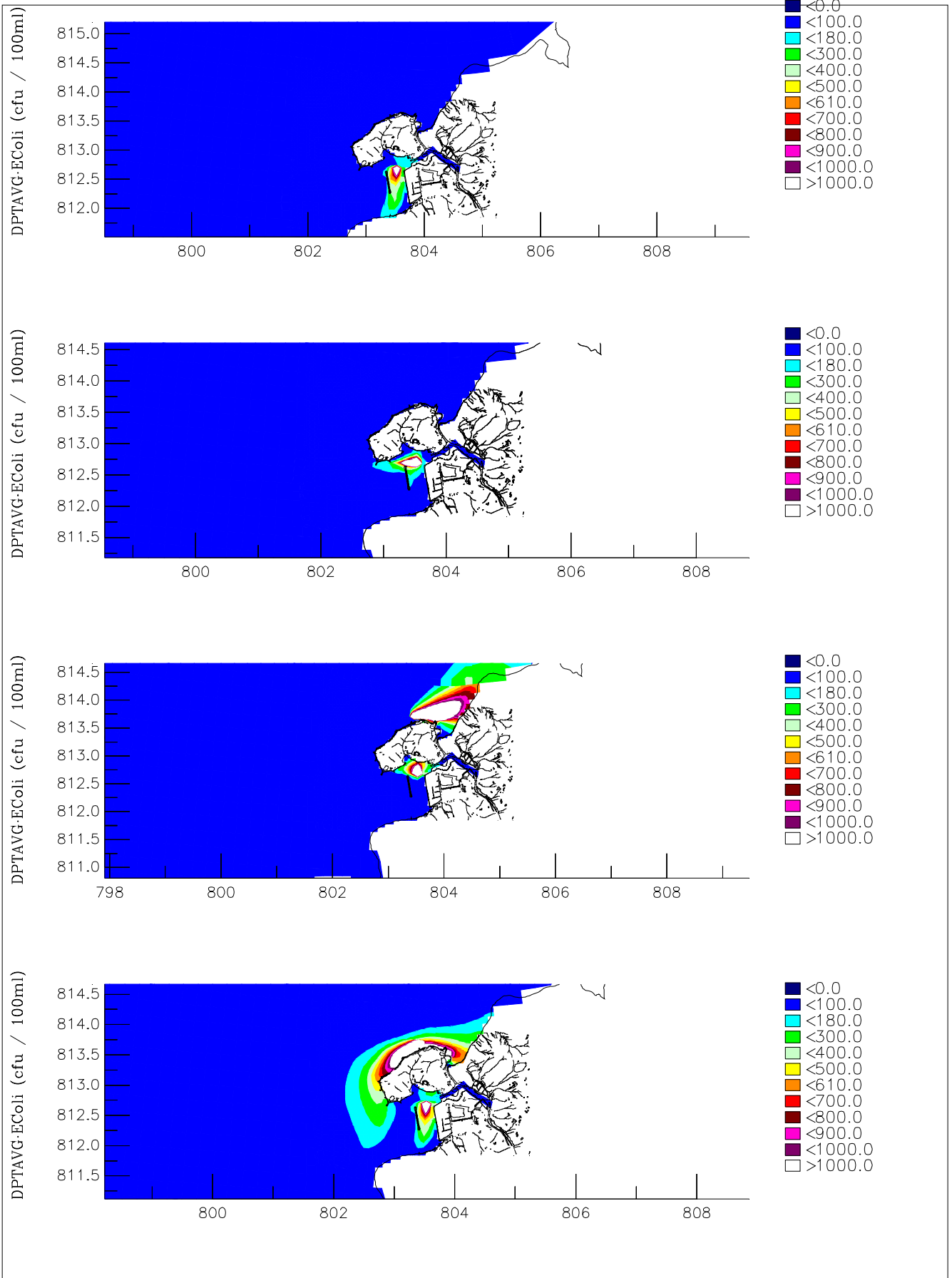
Simulated Depth Averaged EColi 1 hour, 5 hours, 9 hours, 13 hours after Emergency Discharge Dry Season S3d Low Water Slack Tide + Neap Tide DSD & ATKINS Figure 5F-17
