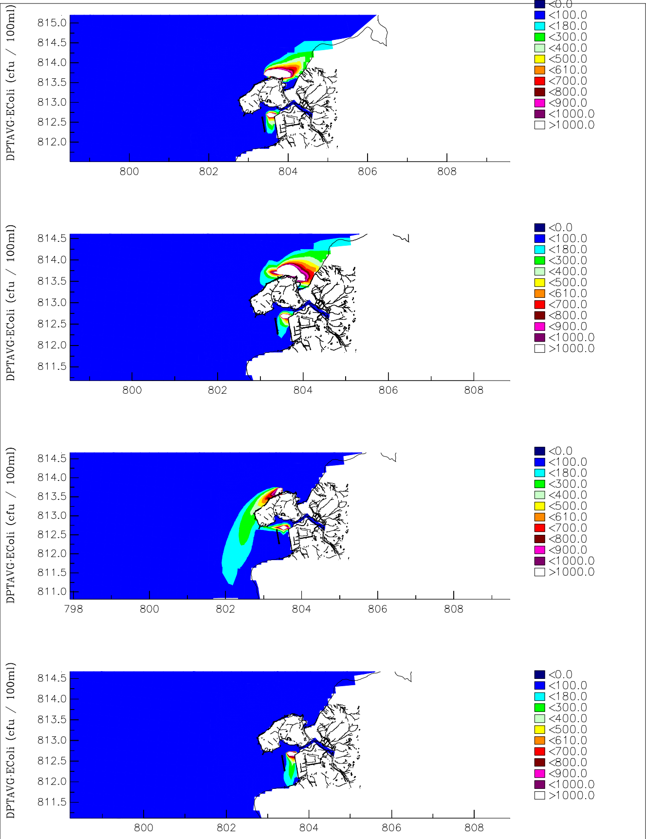
Simulated Depth Averaged EColi 1 hour, 5 hours, 9 hours, 13 hours after Emergency Discharge Wet Season S3h Low Water Slack Tide + Neap Tide DSD & ATKINS Figure 5F-37
