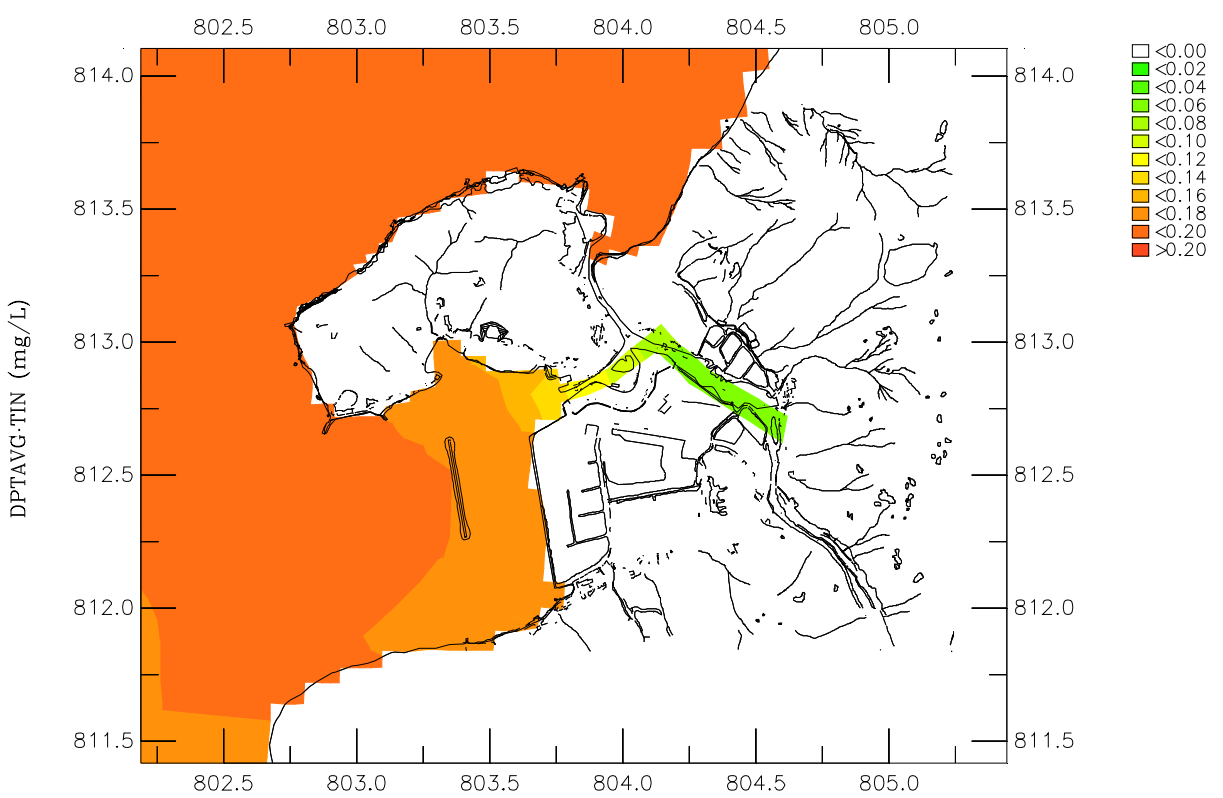
Simulated Depth Averaged TIN Normal Operation (Upper) and Maximum Concentration (Lower) occurred at 15:00 Aug 05 during Emergency Discharge
