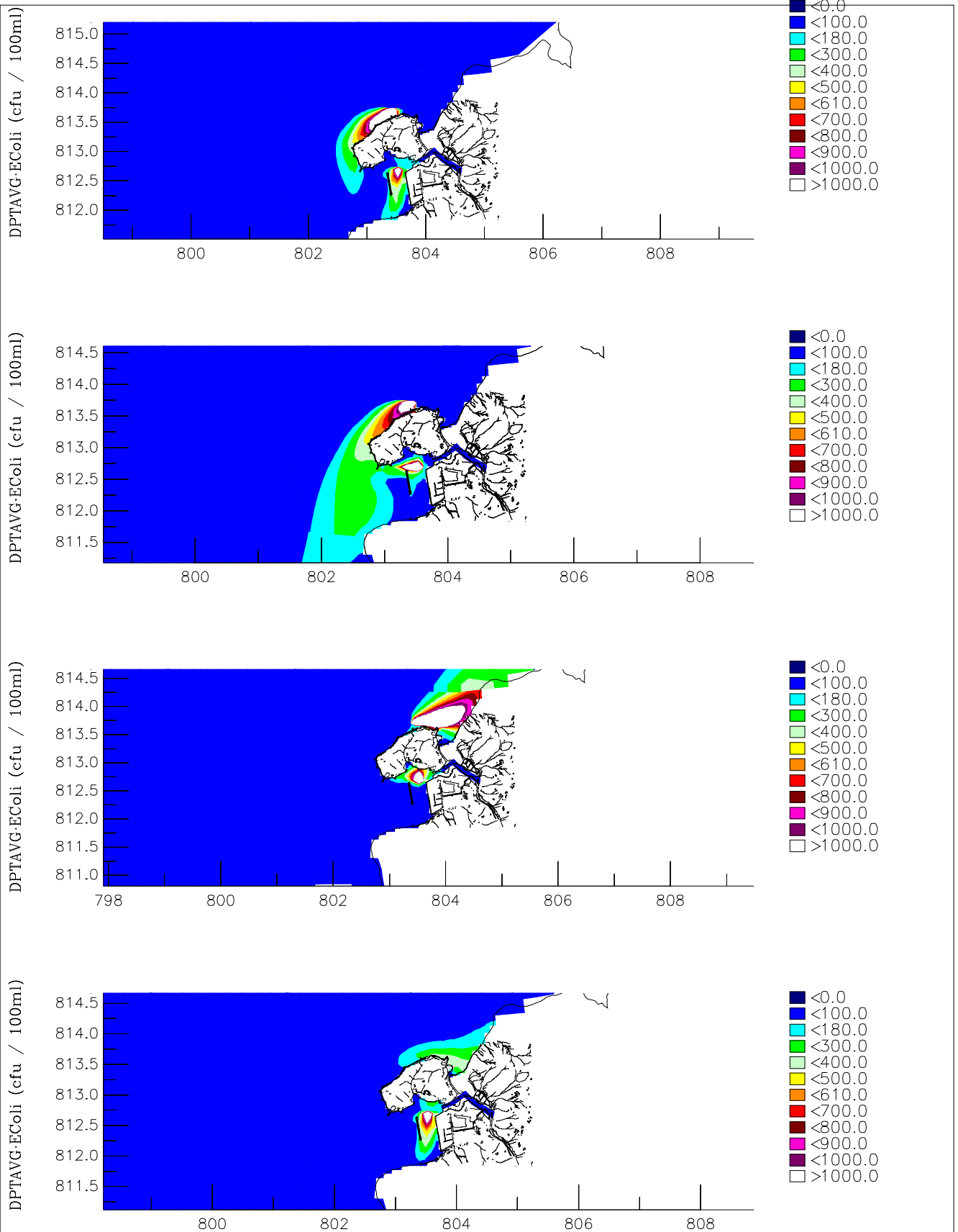
Simulated Depth Averaged EColi 1 hour, 5 hours, 9 hours, 13 hours after Emergency Discharge Dry Season S3c High Water Slack Tide + Neap Tide DSD & ATKINS Figure 5F-12
