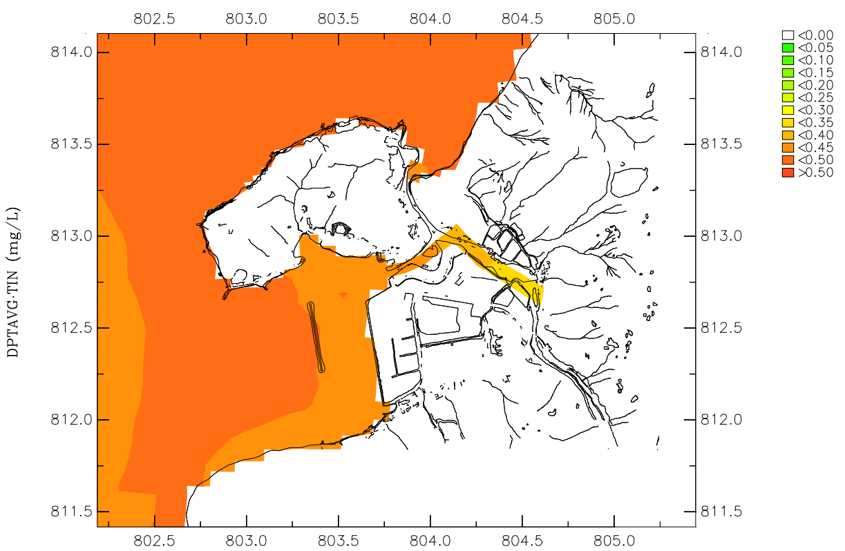
Simulated Depth Averaged TIN Normal Operation (Upper) and Maximum Concentration (Lower) occurred at 08:00 Jul 27 during Emergency Discharge
