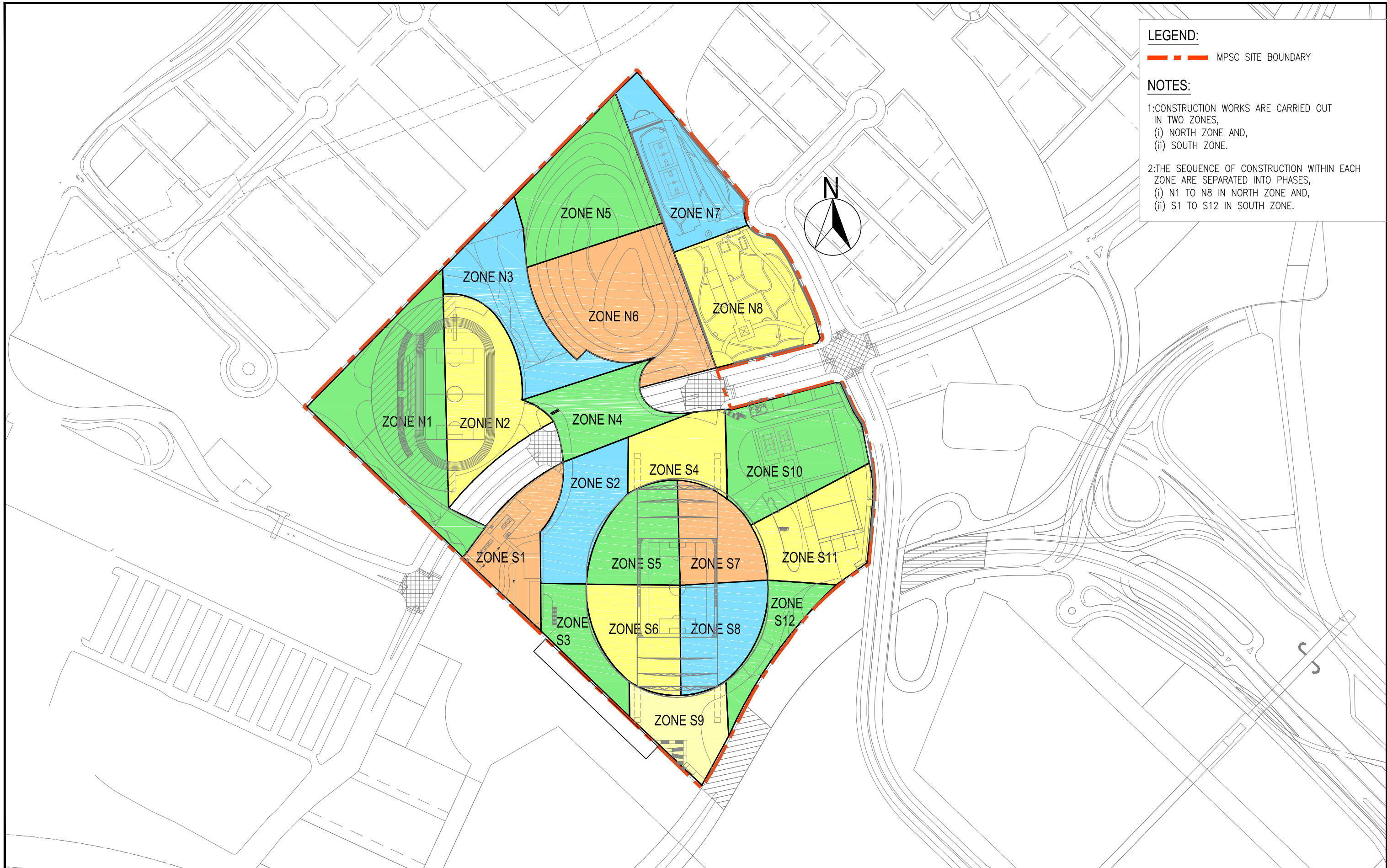
Figure 2-2: CONSTRUCTION PHASING PLAN (SCALE 1:4000)
