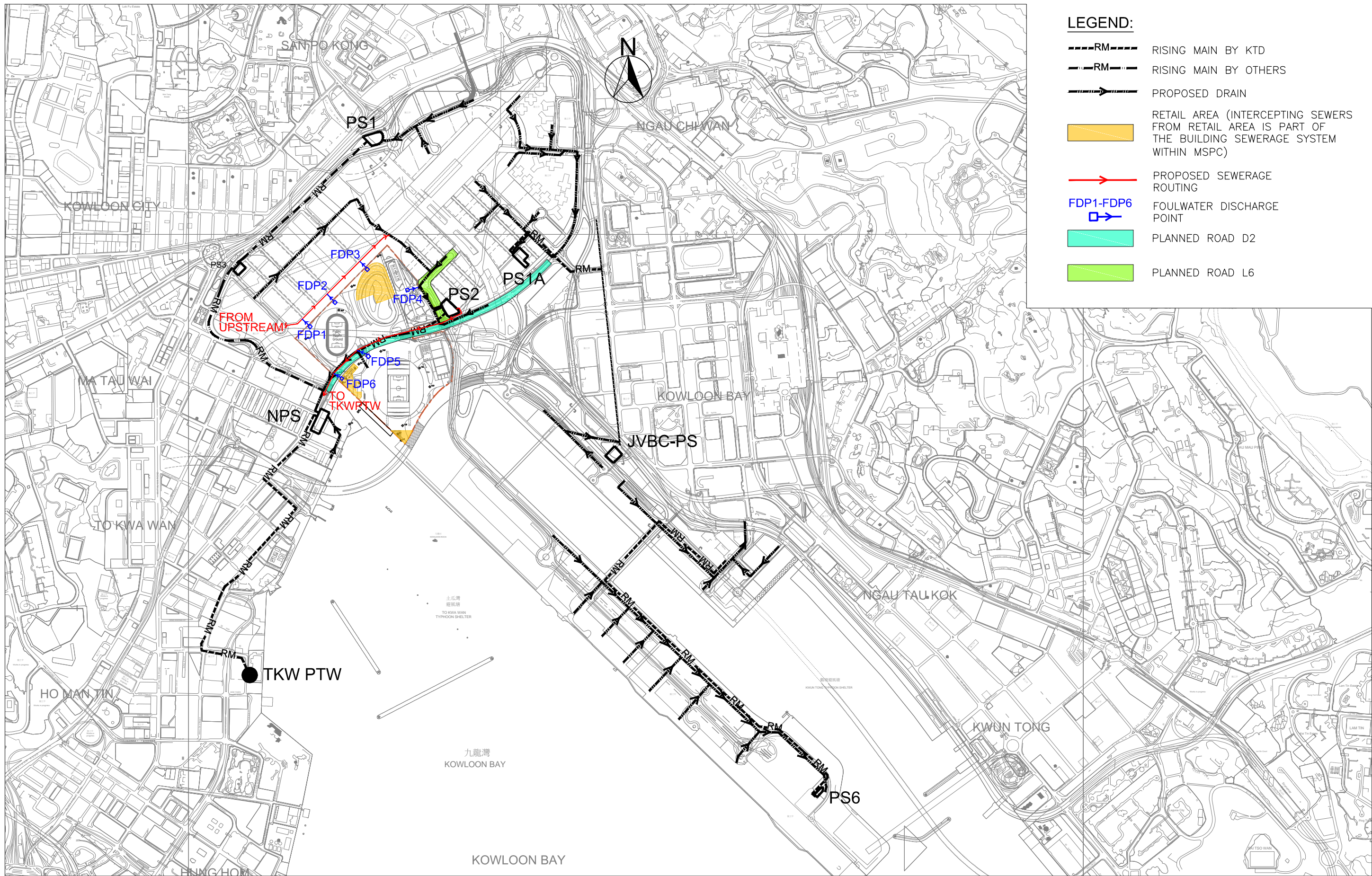
Figure 7-2-1: SEWERAGE LAYOUT PLAN -- KTD (EXTRACT FROM KAI TAK DEVELOPMENT EIA REPORT)
