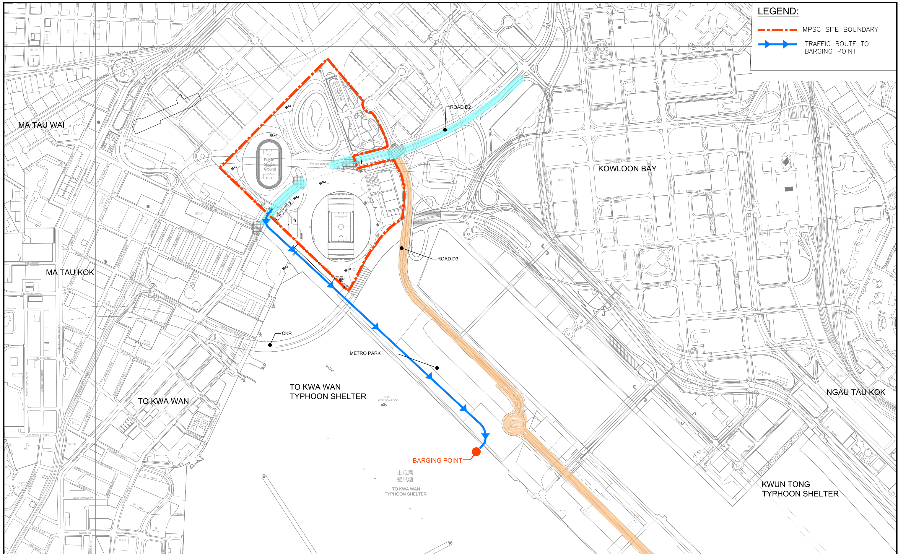
Figure 8-3-2: TRAFFIC ROUTE TO BARGING POINT WHEN ROAD D2 & D3 IS NOT AVAILABLE (SCALE 1:8000)
