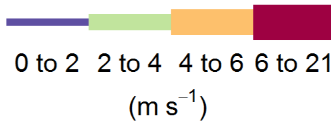
Frequency of counts by wind direction (%)
