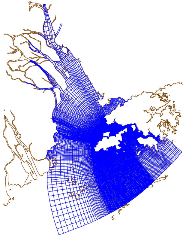
Grid Layout and Model Coverage
