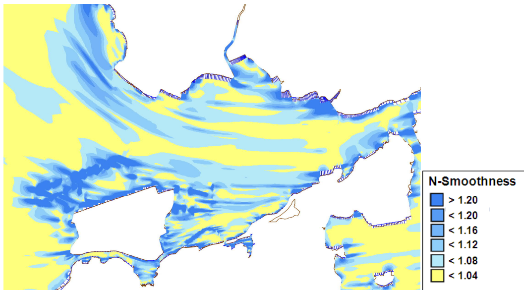
N-Smoothness of Detailed Model Grid
