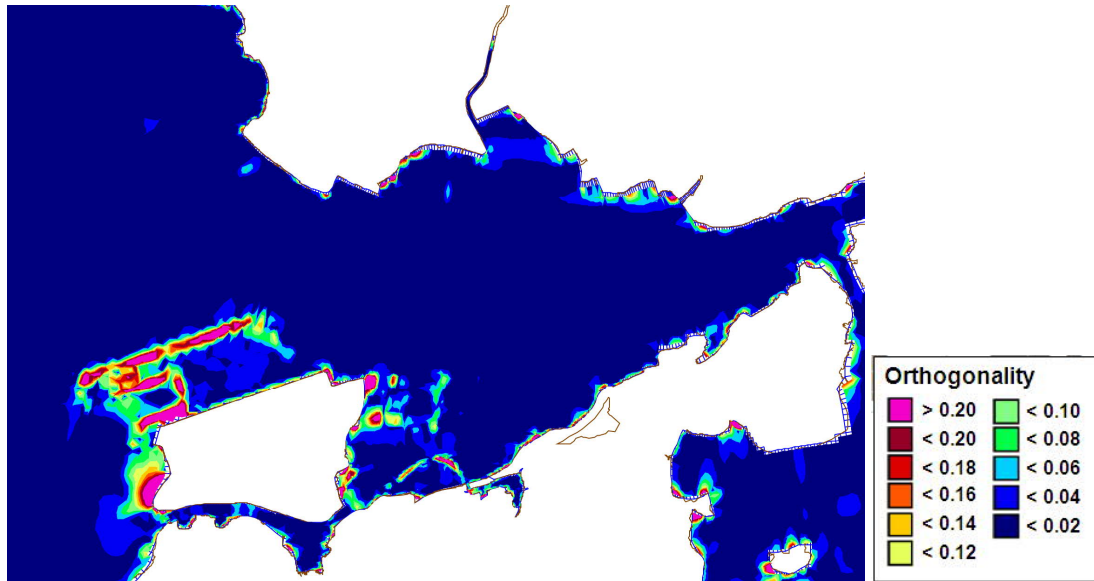
Orthogonality of Detailed Model Grid
