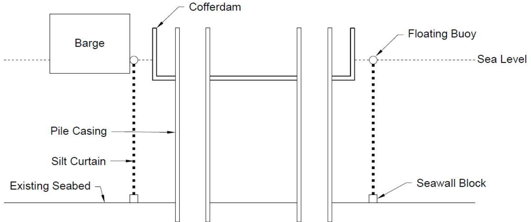
Schematic Diagram of Cofferdam and Steel Pile Casing with Silt Curtain
