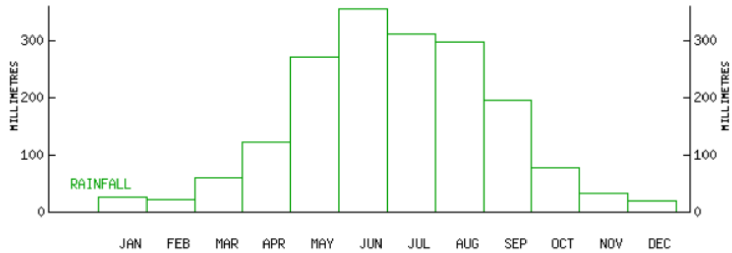
Figure 1 Rainfall Statistics (mm) for Tai Po (Monthly means for 2000 to 2018)
