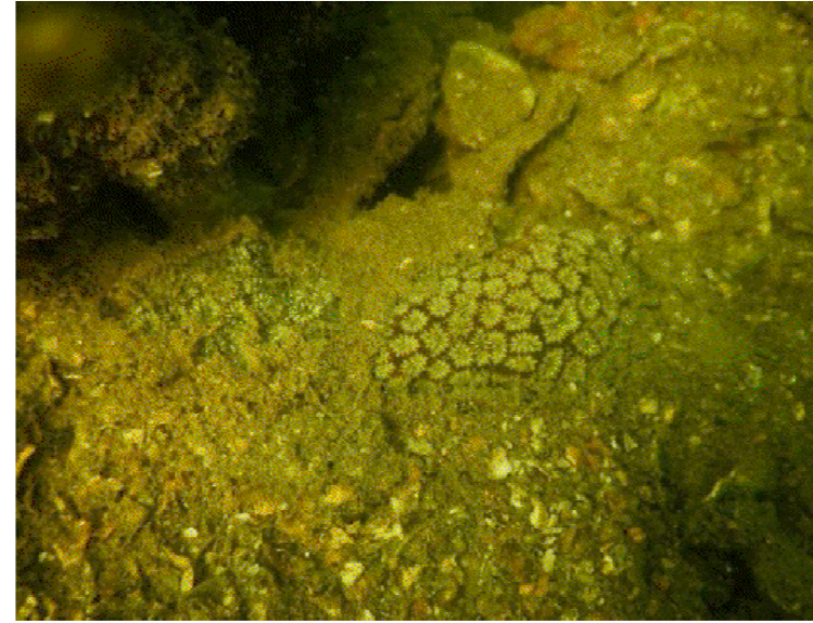
Oulastrea crispata (at Seawall)
