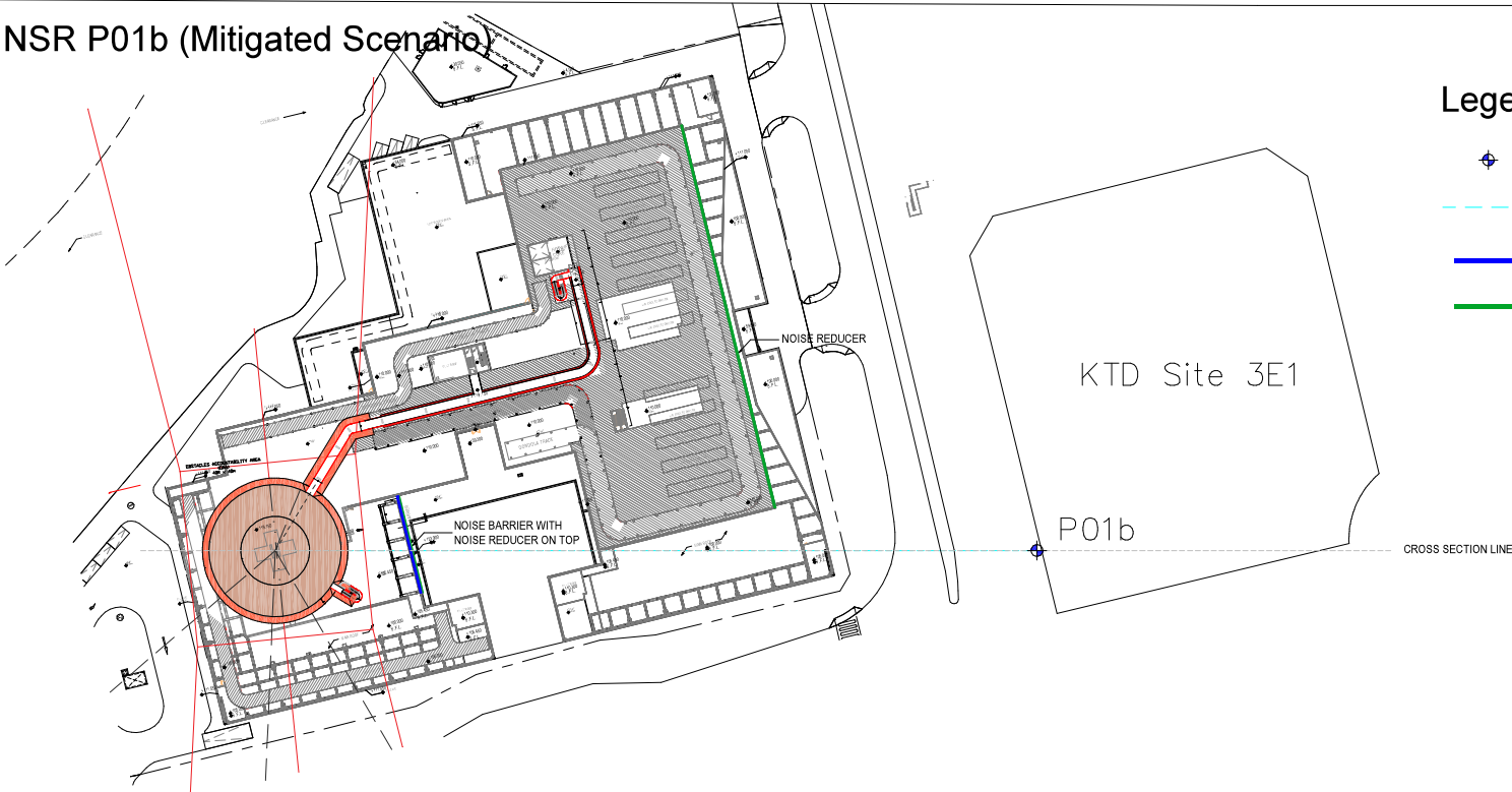
PLAN VIEW
