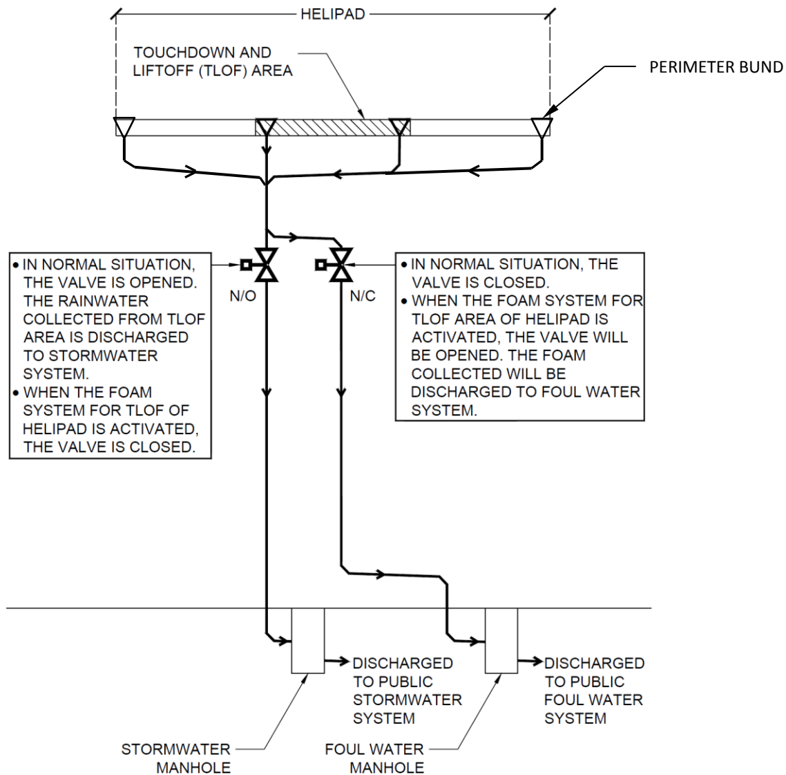
NAH - DRAINAGE SYSTEM FOR TLOF AREA OF HELIPAD
