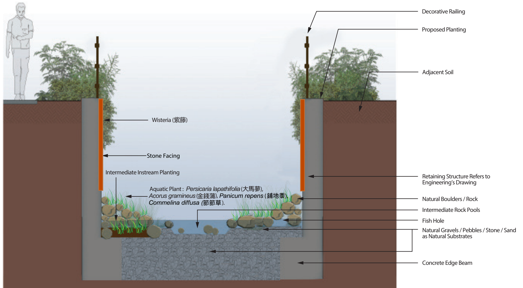
Rectangular Green Channel : Concrete Rectangular Channel with Natural Bedding and Natural Rock TYPICAL SECTION A-A AT NATURAL BED LOCATION
