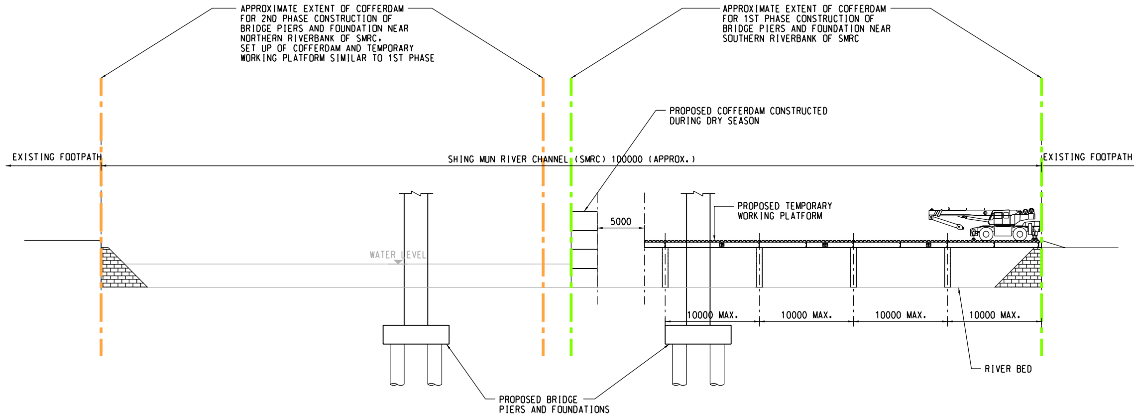
SECTION A - A TYPICAL SECTION OF TEMPORARY WORKING PLATFORM
