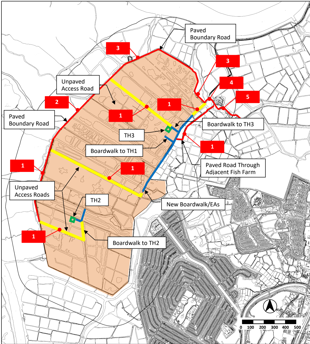
Figure 4-4 Noise Emission Sources Within the Project Site
