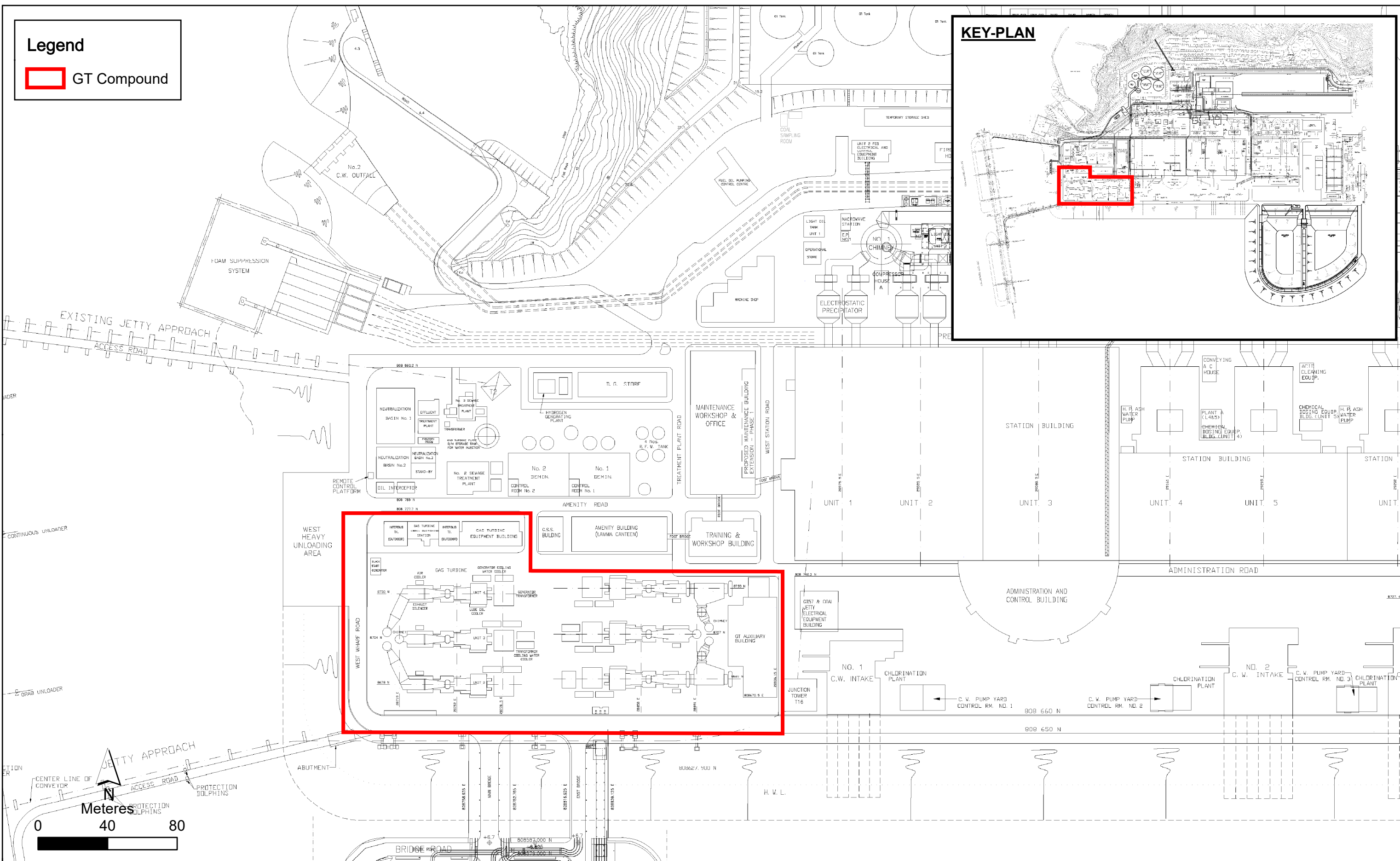
Figure 1.1 Location of Gas Turbine Compound at Lamma Power Station
