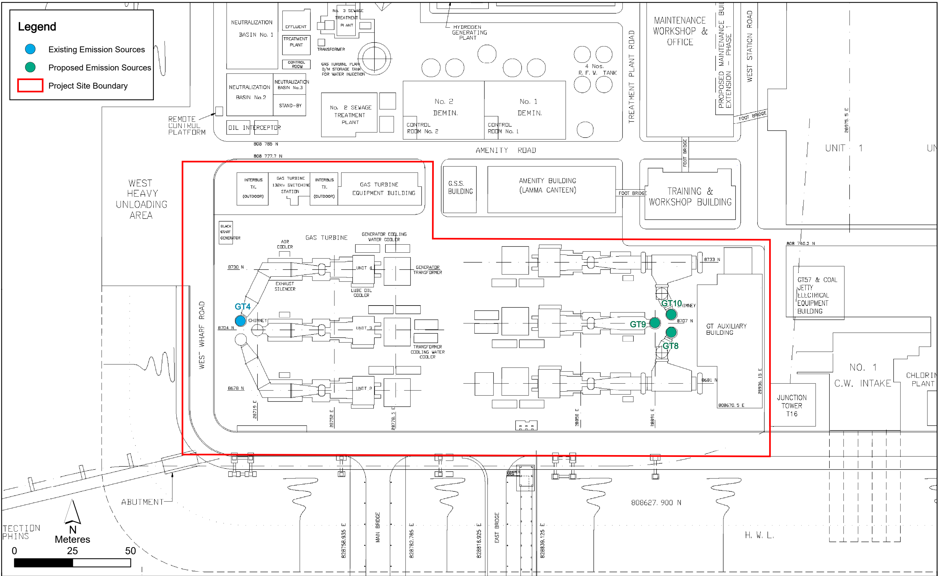
Figure 3.4c Locations of Emission Sources within the Gas Turbine Compound ("With Project" Scenario - Phase 3)
