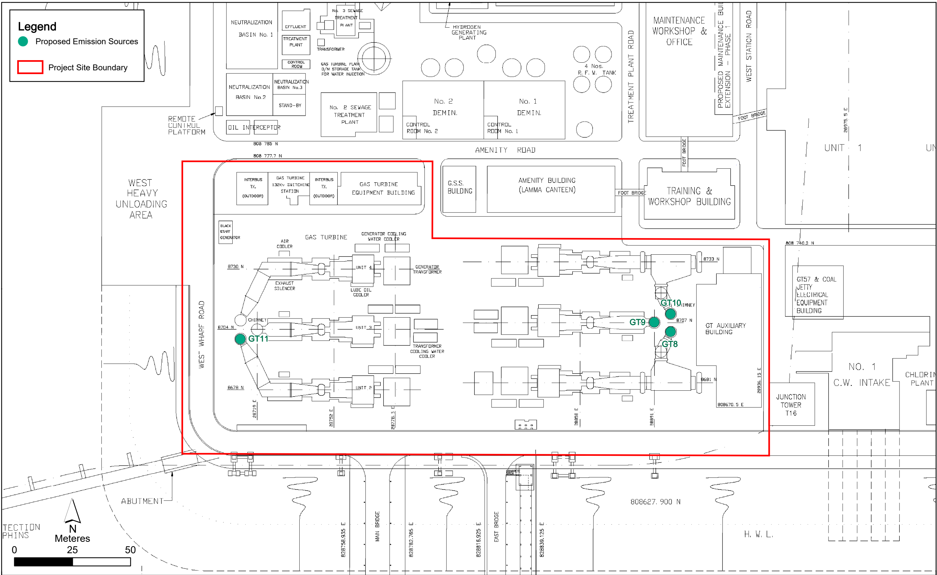
Figure 3.4d Locations of Emission Sources within the Gas Turbine Compound ("With Project" Scenario - Phase 4)
