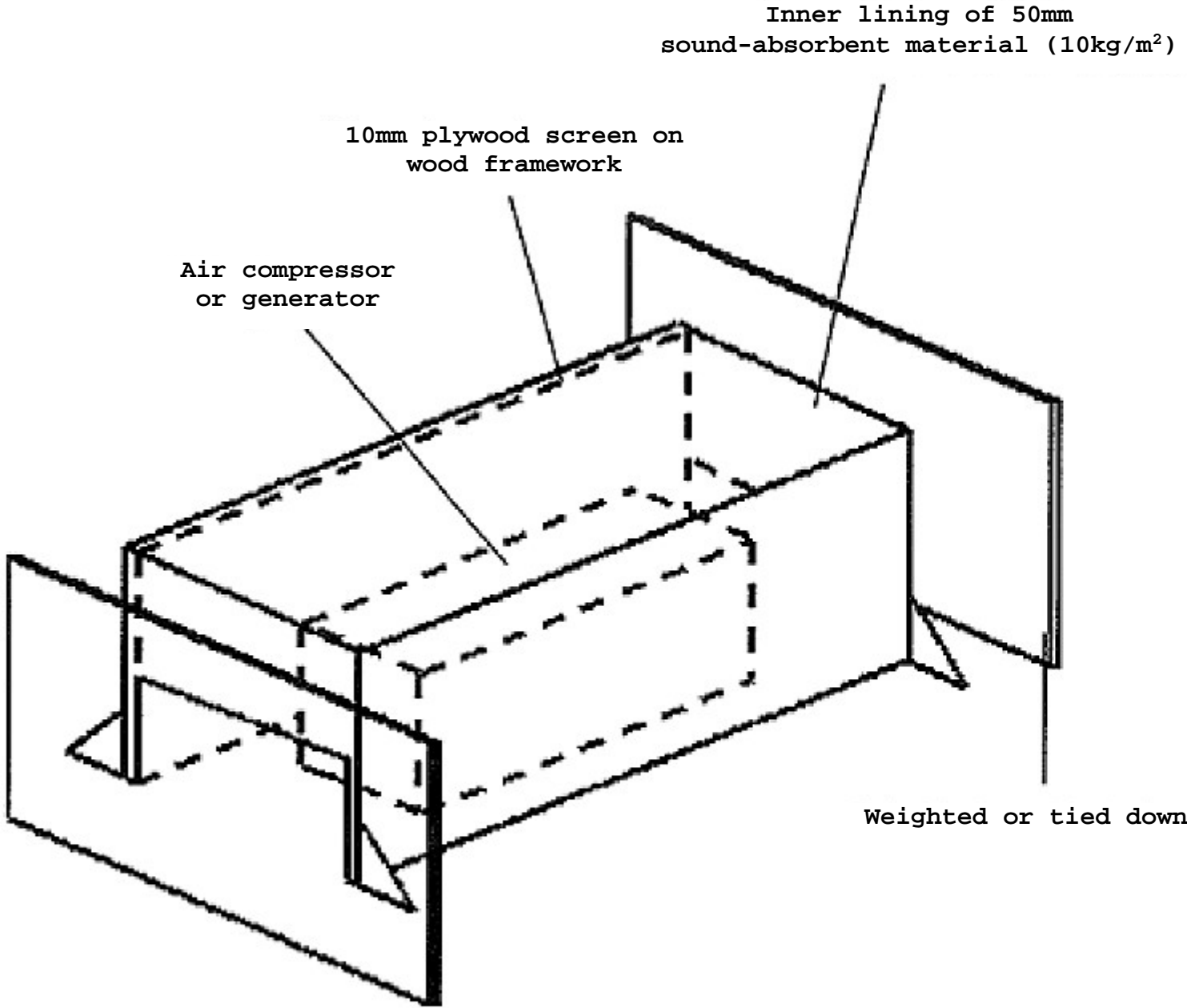
Typical Noise Enclosure for Static Plant (e.g. Air Compressors, Generators etc.) ~3-4m tall
