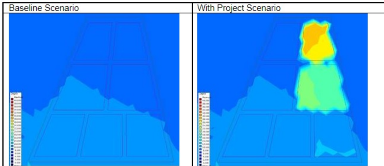
Figure 3.4 Modelled Bathymetry
