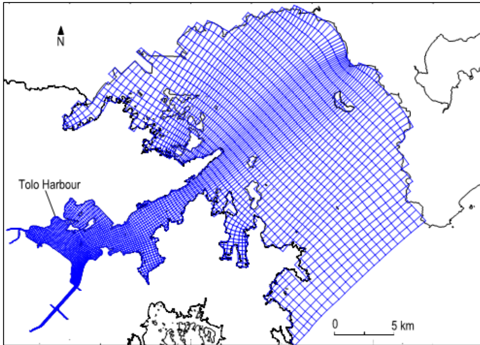
THMB Model Grid Layout – Overview
