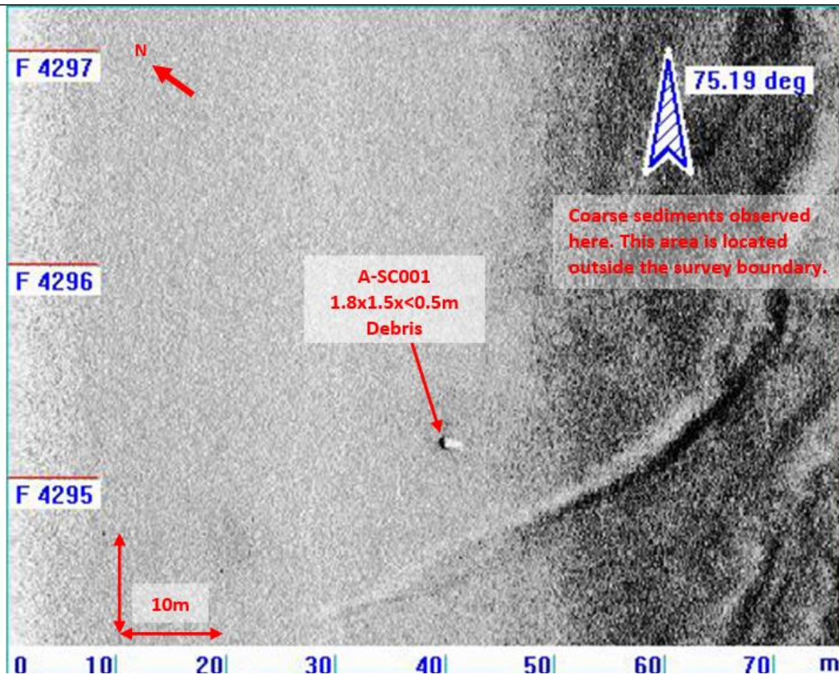
Figure 9.3 SSS Rectified Image Showing Sonar Contact A-SC001
